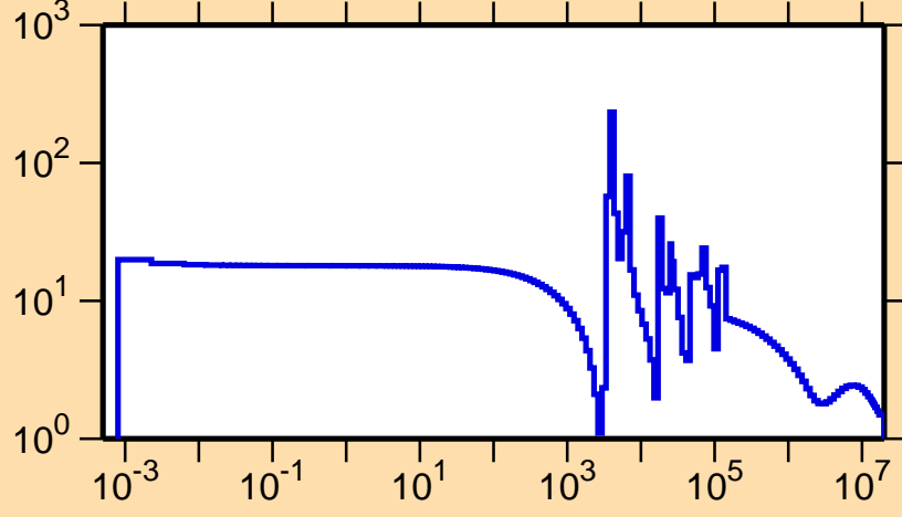
\sigma vs. E for ^{81}\text{Ga}(n,\text{el.})
