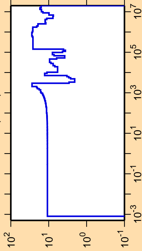
\Delta\sigma/\sigma vs. E for ^{81}\text{Ga}(n,\text{el.})
