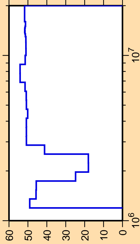
\Delta\sigma/\sigma vs. E for ^{81}\text{Ga}(n,n_3)
