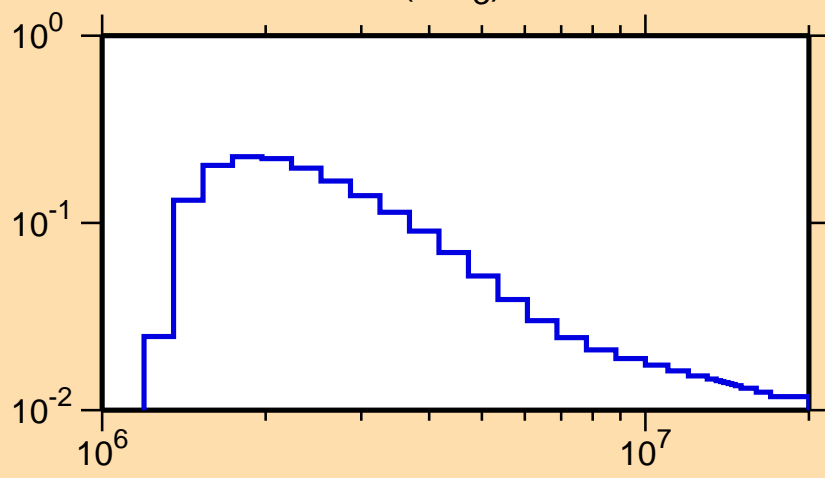
\sigma vs. E for ^{81}\text{Ga}(n,n_3)
