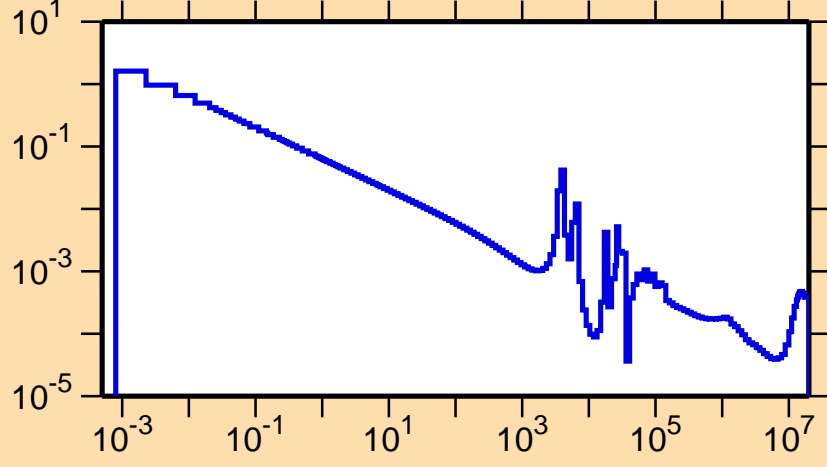
\sigma vs. E for ^{81}\text{Ga}(n,\gamma)
