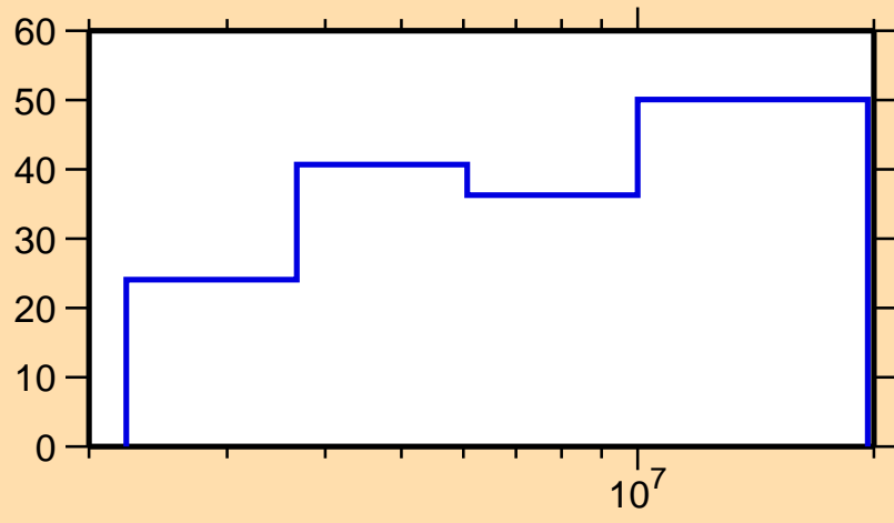
\Delta\sigma/\sigma vs. E for ^{81}\text{Ga}(n,n_1)
