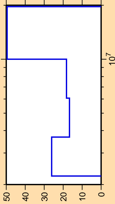
\Delta\sigma/\sigma vs. E for ^{81}\text{Ga}(n,n\text{cont.})
