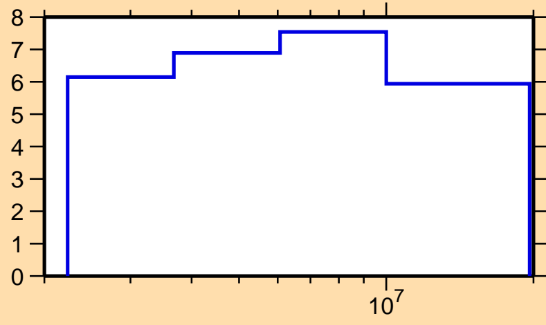
\Delta\sigma/\sigma vs. E for ^{81}\text{Ga}(n,n\text{onel.})
