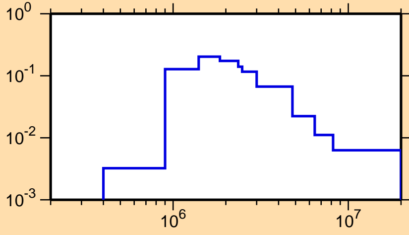
\sigma vs. E for ^{81}\text{Ga}(n,n_2)
