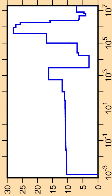
\Delta\sigma/\sigma vs. E for ^{81}\text{Ga}(n,\text{tot.})
