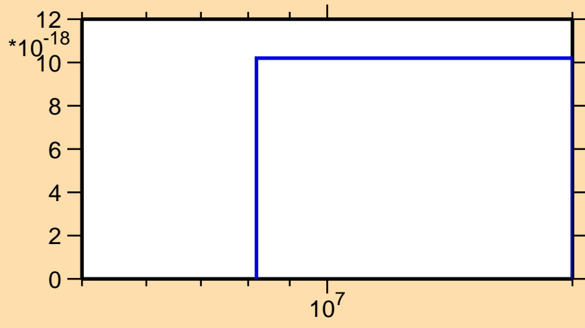
\sigma vs. E for ^{81}\text{Ga}(n,2np)
