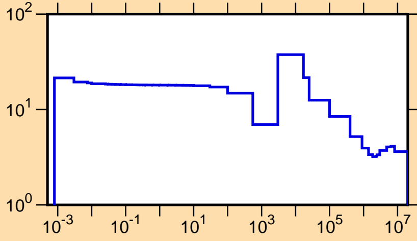
\sigma vs. E for ^{81}\text{Ga}(n,\text{tot.})
