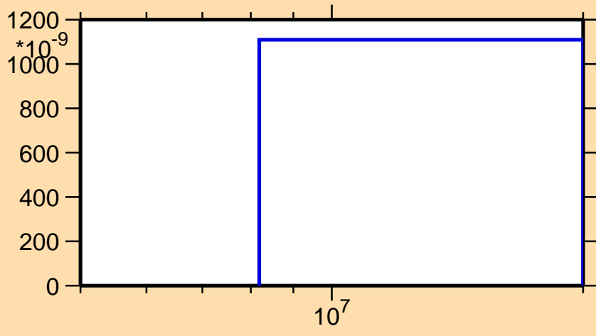
\sigma vs. E for ^{81}\text{Ga}(n,\alpha)
