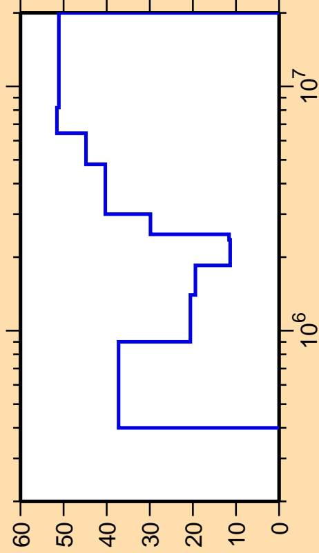
\Delta\sigma/\sigma vs. E for ^{81}\text{Ga}(n,n_2)
