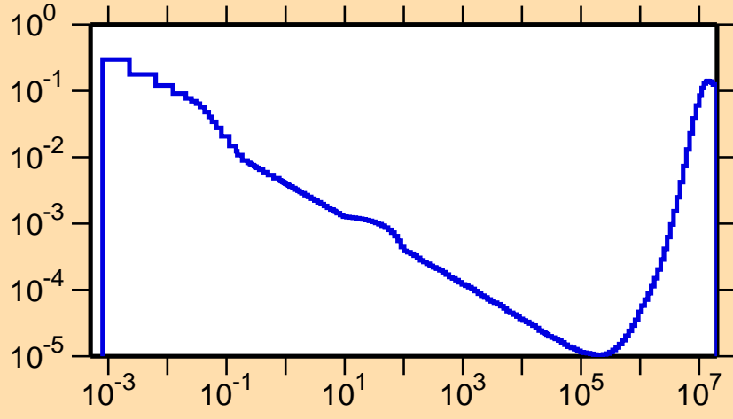
\sigma vs. E for ^{135}\text{Gd}(n,p\alpha)
