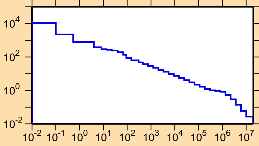
\sigma vs. E for ^{135}\text{Gd}(n,p)
