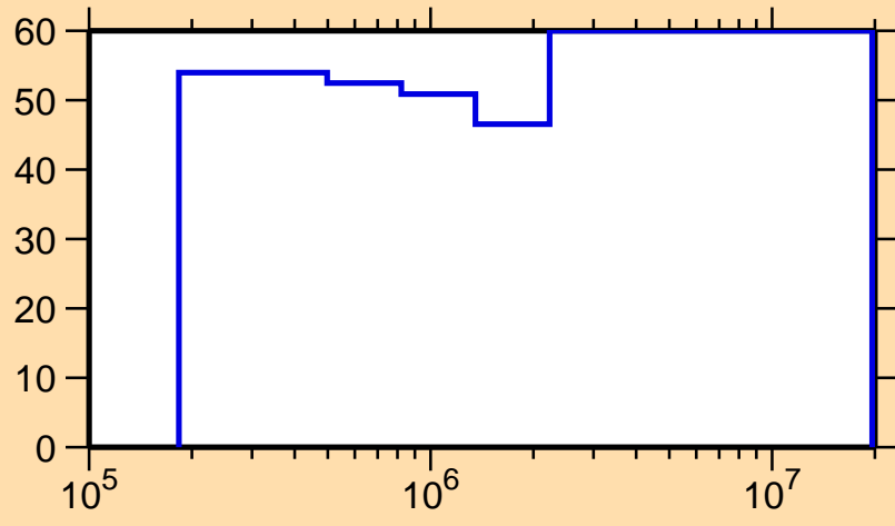
\Delta\sigma/\sigma vs. E for ^{135}\text{Gd}(n,n_1)
