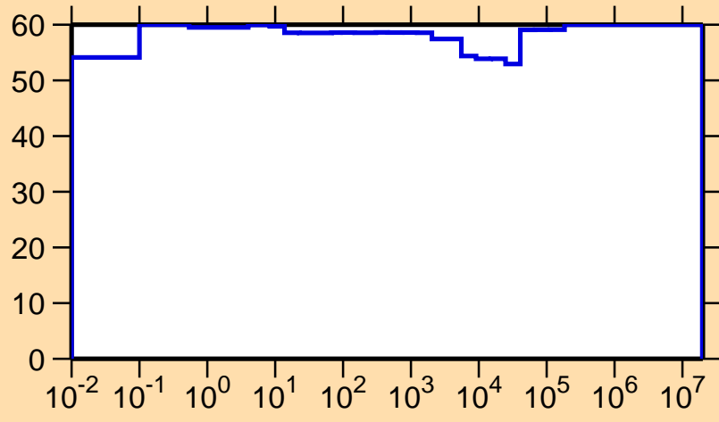
\Delta\sigma/\sigma vs. E for ^{135}\text{Gd}(n,p)
