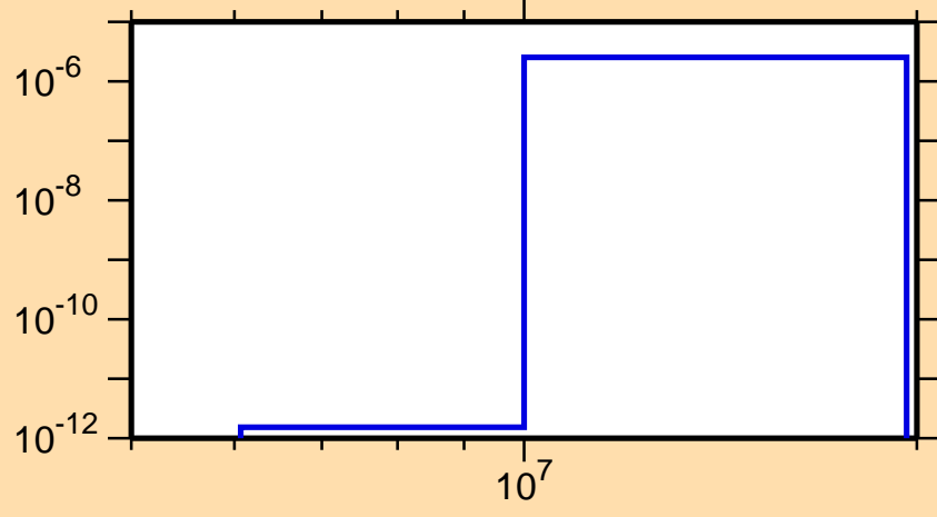
\sigma vs. E for ^{135}\text{Gd} (mt 45)
