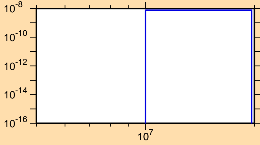
\sigma vs. E for ^{135}\text{Gd}(\text{mt } 34)
