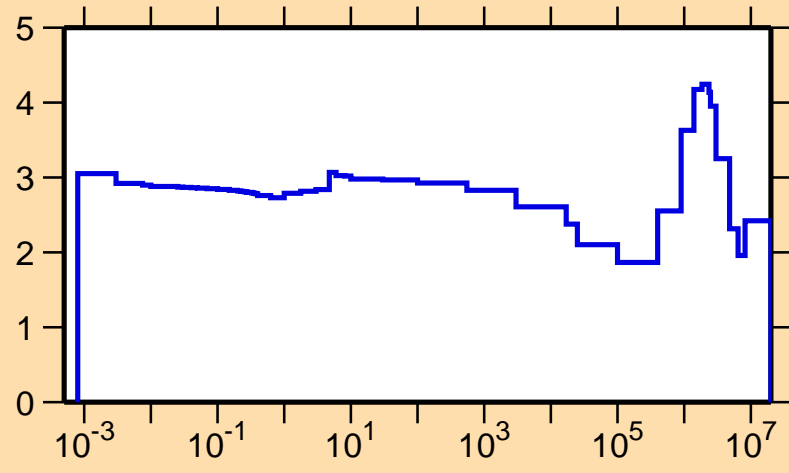
\sigma vs. E for ^{135}\text{Gd}(n,\text{el.})
