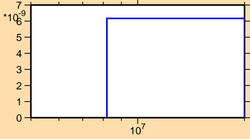
\sigma vs. E for ^{135}\text{Gd} (mt 34)
