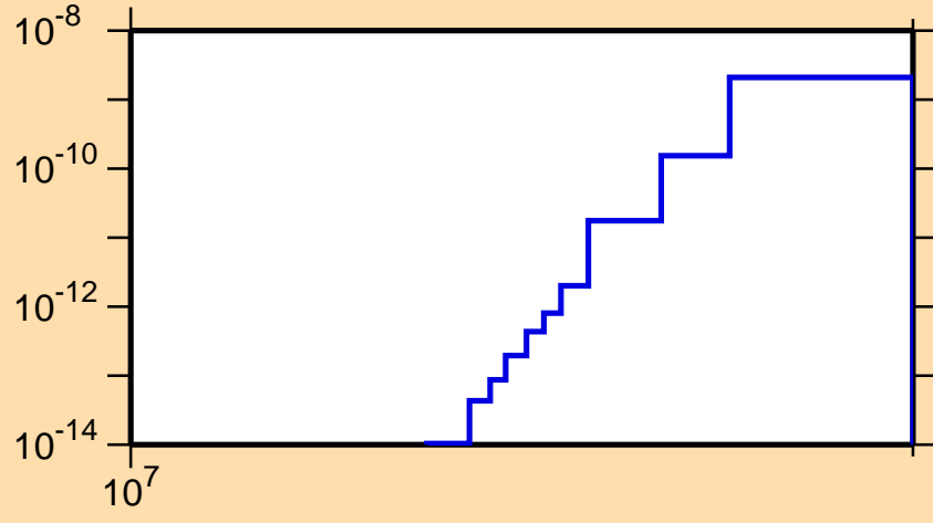
\sigma vs. E for ^{136}\text{Gd}(\text{mt } 34)
