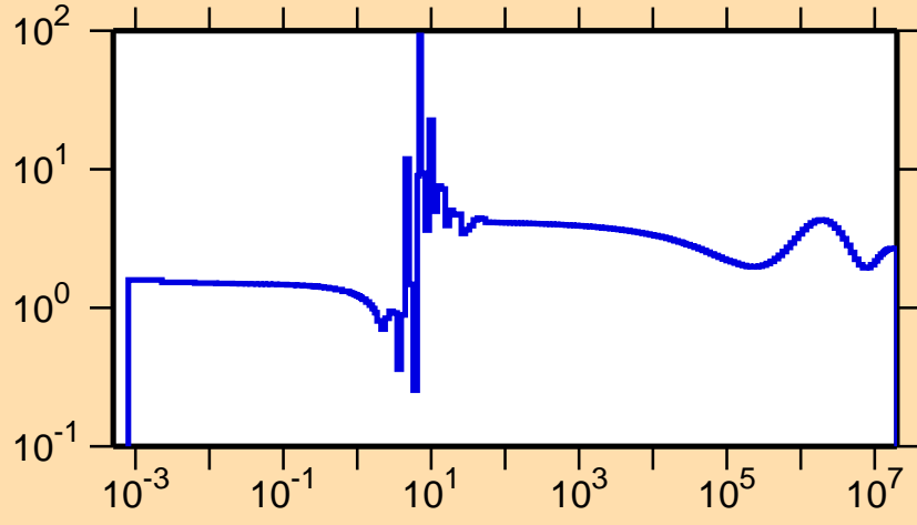
\sigma vs. E for ^{136}\text{Gd}(n,\text{el.})
