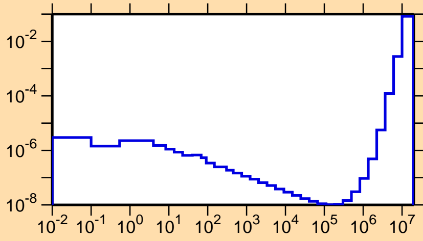
\sigma vs. E for ^{136}\text{Gd}(n,p\alpha)
