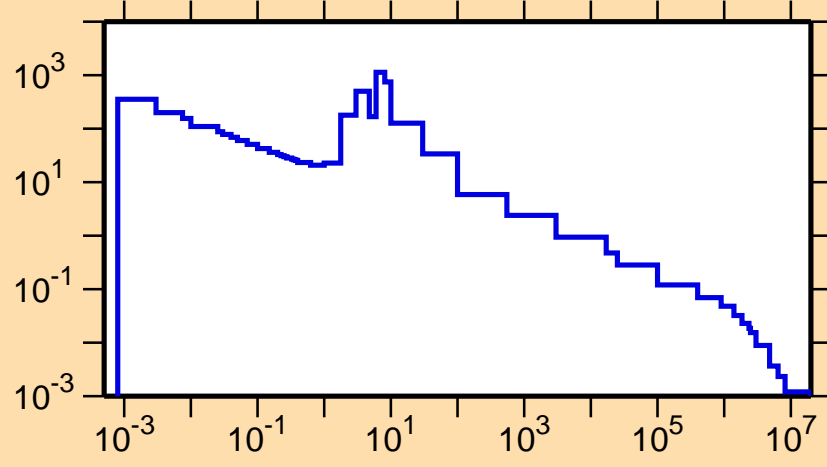
\sigma vs. E for ^{136}\text{Gd}(n,\gamma)
