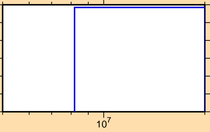
\sigma vs. E for ^{136}\text{Gd}(n,2n)
