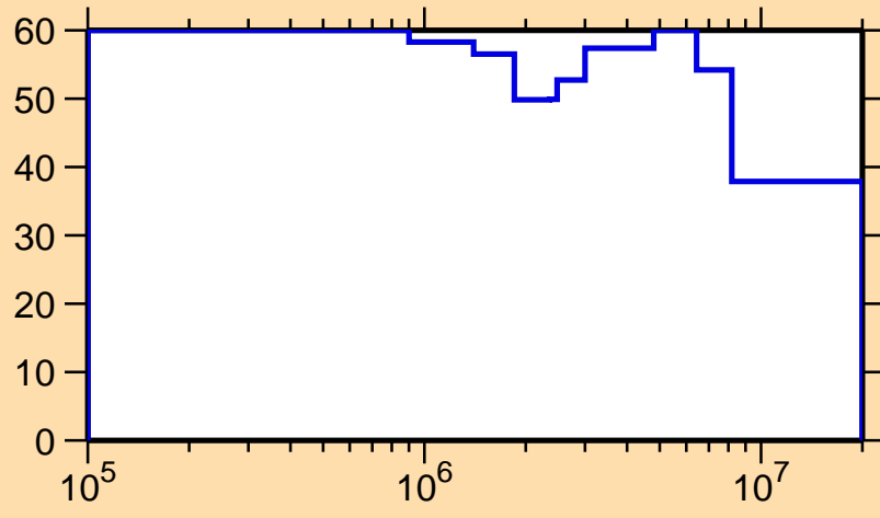
\Delta\sigma/\sigma vs. E for ^{136}\text{Gd}(n,n_1)
