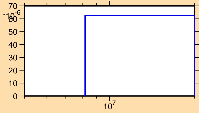
\sigma vs. E for ^{136}\text{Gd}(n,t)
