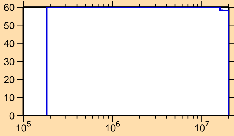
\Delta\sigma/\sigma vs. E for ^{137}\text{Gd}(n,ncont.)
