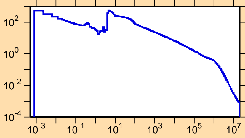
\sigma vs. E for ^{137}\text{Gd}(n,\gamma)
