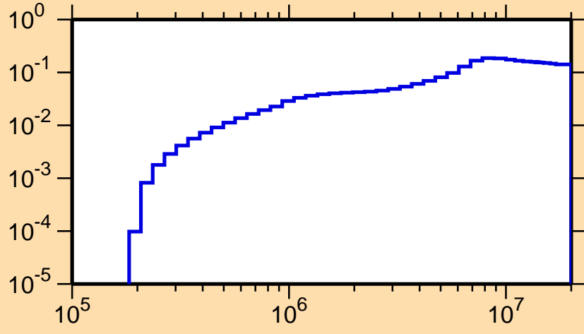
\sigma vs. E for ^{137}\text{Gd}(n,n\text{cont.})
