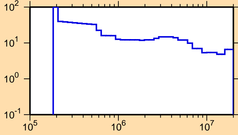
\Delta\sigma/\sigma vs. E for ^{137}\text{Gd}(n,\text{el.})
