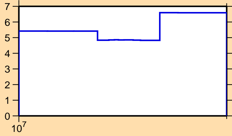
\Delta\sigma/\sigma vs. E for ^{137}\text{Gd}(n,\text{el.})
