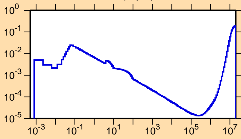
\sigma vs. E for ^{137}\text{Gd}(n,p\alpha)
