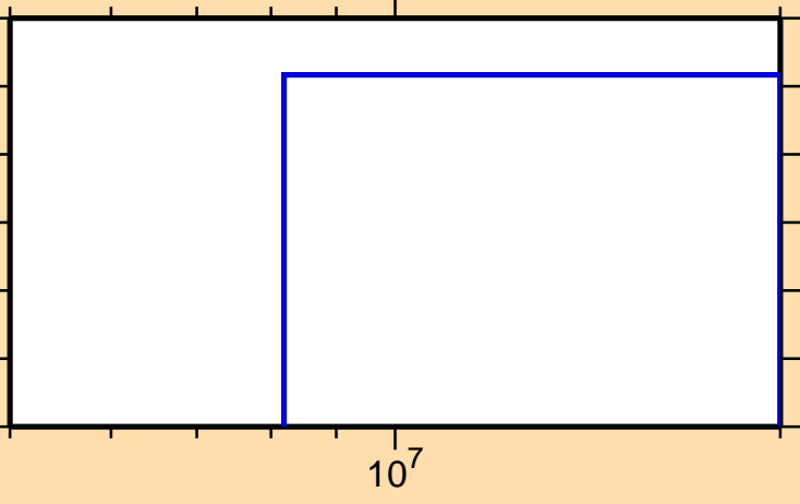
\sigma vs. E for ^{137}\text{Gd} (mt 34)
