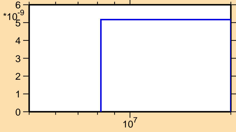
\sigma vs. E for ^{137}\text{Gd} (mt 34)
