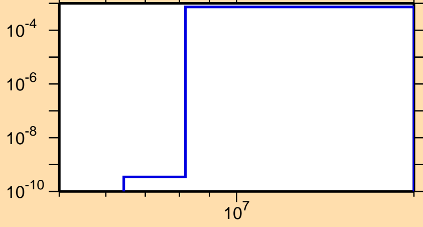
\sigma vs. E for ^{137}\text{Gd}(n,\text{pd})
