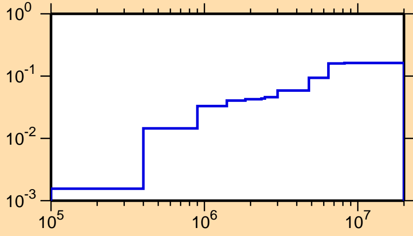
\sigma vs. E for ^{137}\text{Gd}(n,\text{inel.})
