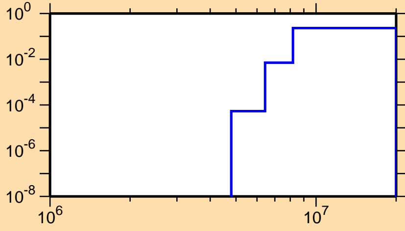
\sigma vs. E for ^{137}\text{Gd}(n,np)
