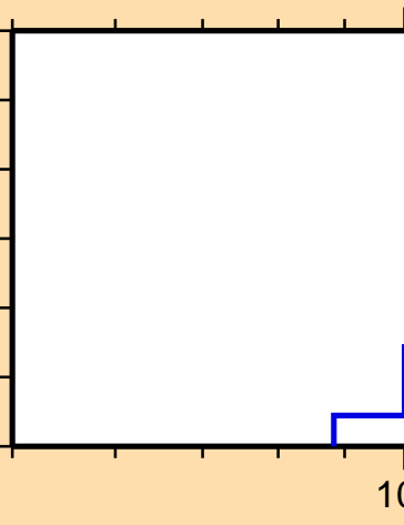
\sigma vs. E for ^{138}\text{Gd}(\text{mt117})
