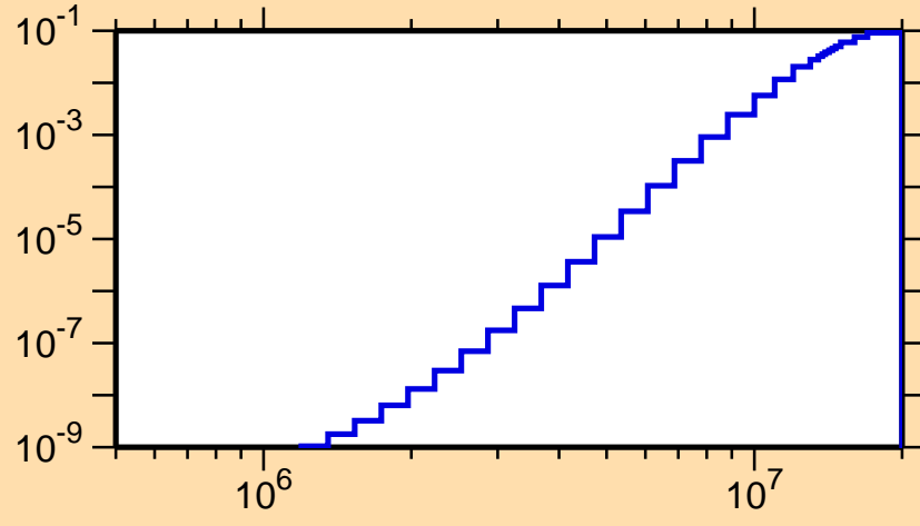
\sigma vs. E for ^{138}\text{Gd}(n,p\alpha)
