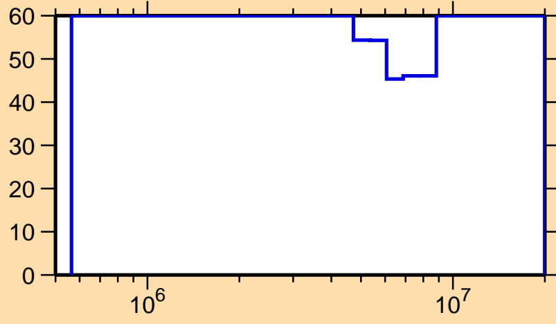
\Delta\sigma/\sigma vs. E for ^{138}\text{Gd}(n,n\text{cont.})
