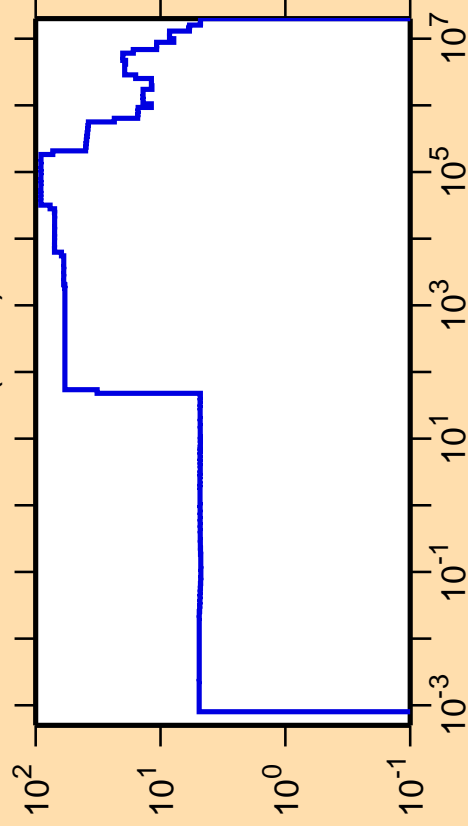
\Delta\sigma/\sigma vs. E for ^{138}\text{Gd}(n,\text{el.})
