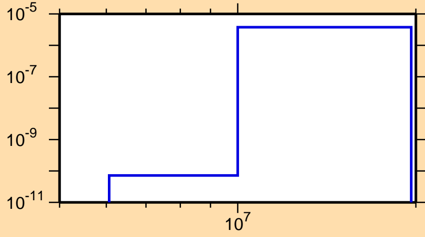
\sigma vs. E for ^{138}\text{Gd} (mt 45)
