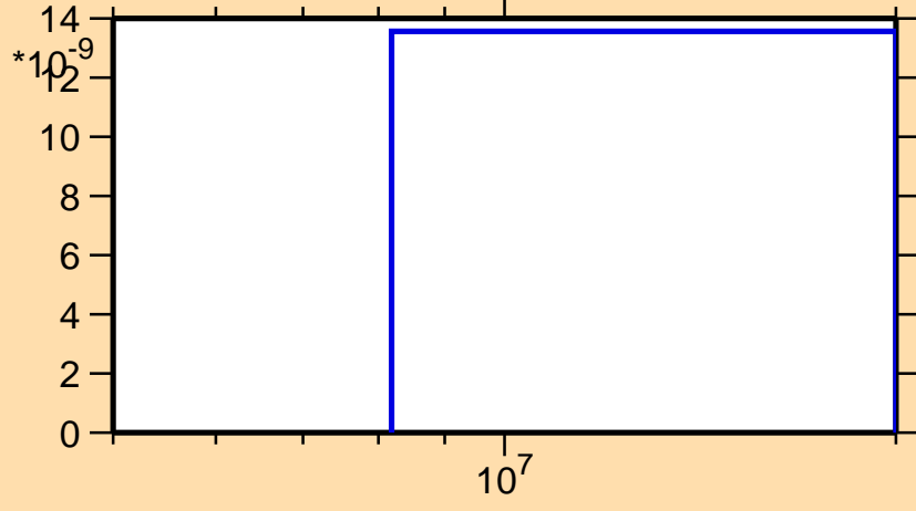
\sigma vs. E for ^{138}\text{Gd}(\text{mt117})
