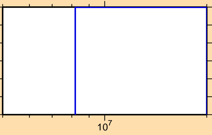
\sigma vs. E for ^{138}\text{Gd}(n,2np)
