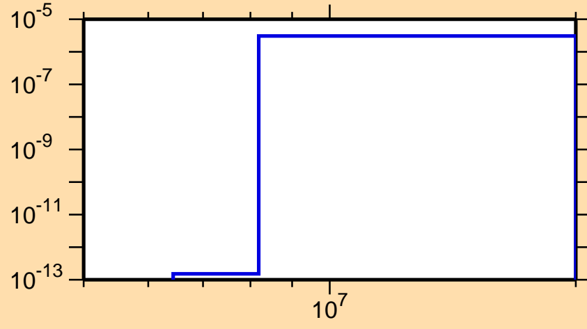
\sigma vs. E for ^{138}\text{Gd}(\text{mt } 45)
