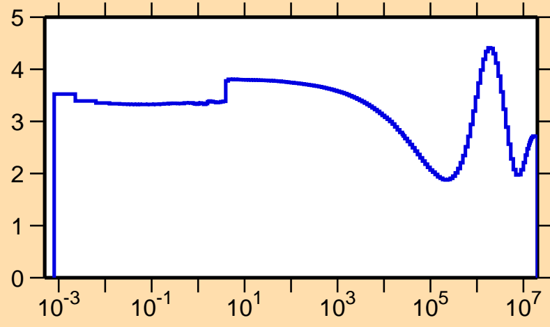
\sigma vs. E for ^{139}\text{Gd}(n,\text{el.})
