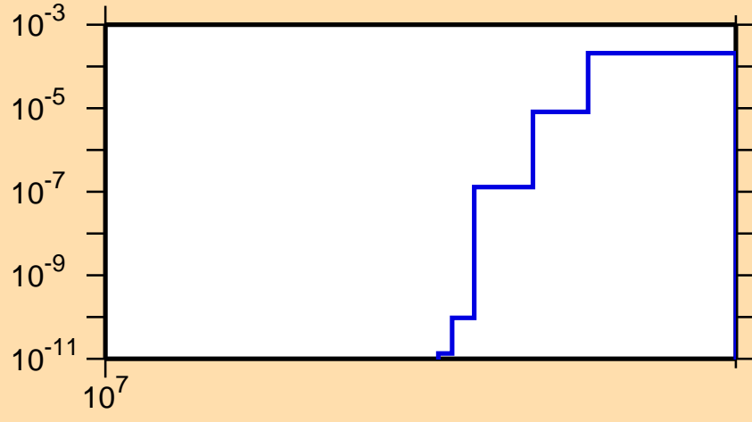
\sigma vs. E for ^{139}\text{Gd}(n,2np)
