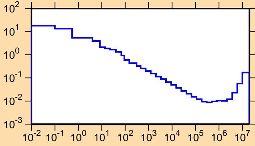
\sigma vs. E for ^{139}\text{Gd}(n,\alpha)
