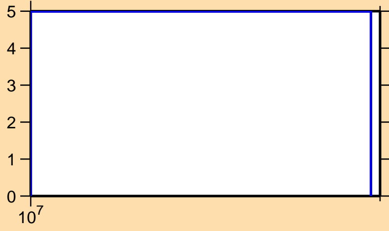
\Delta\sigma/\sigma vs. E for ^{139}\text{Gd}(n,\text{el.})
