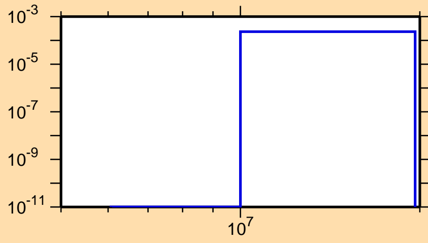
\sigma vs. E for ^{139}\text{Gd}(n,t)
