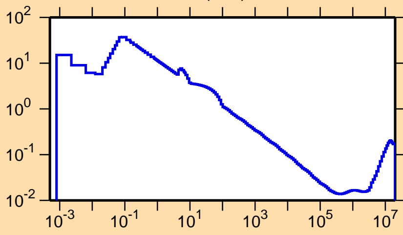
\sigma vs. E for ^{139}\text{Gd}(n,\alpha)
