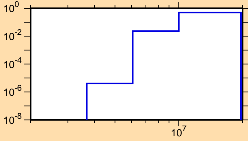
\sigma vs. E for ^{139}\text{Gd}(n,np)
