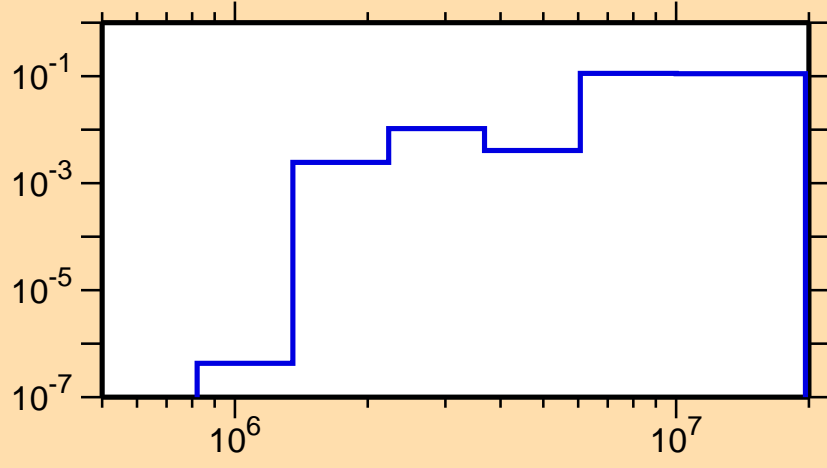
\sigma vs. E for ^{140}\text{Gd}(n,n\text{cont.})
