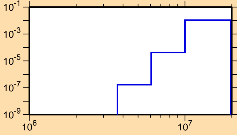
\sigma vs. E for ^{140}\text{Gd}(n,p\alpha)
