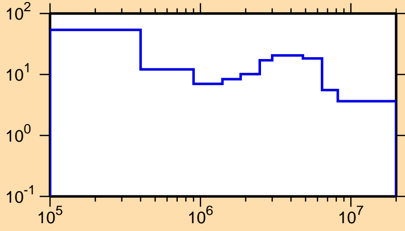
\Delta\sigma/\sigma vs. E for ^{140}\text{Gd}(n,\text{el.})
