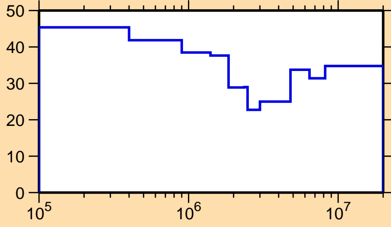
\Delta\sigma/\sigma vs. E for ^{140}\text{Gd}(n,n_1)
