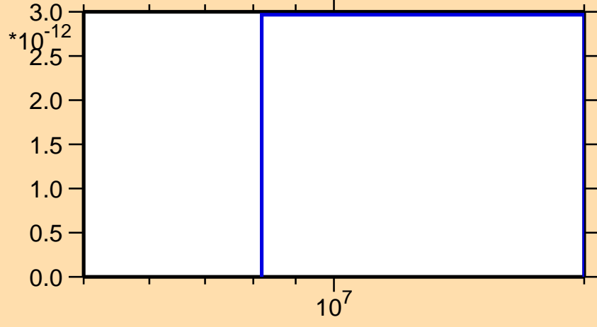
\sigma vs. E for ^{140}\text{Gd} (mt 34)
