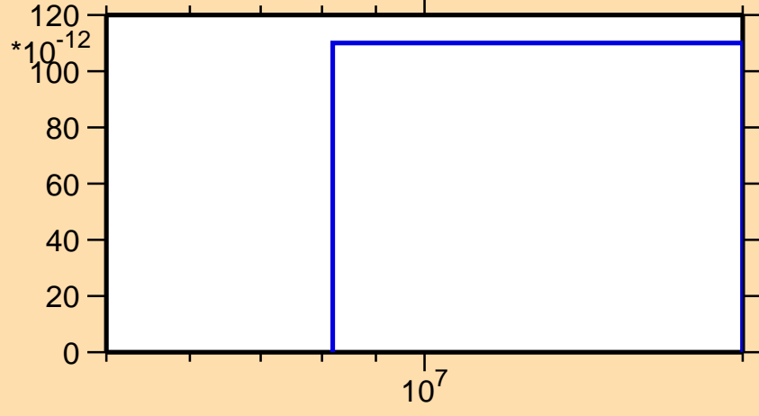
\sigma vs. E for ^{140}\text{Gd}(n,\text{nd})
