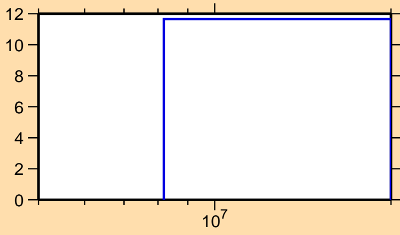
\Delta\sigma/\sigma vs. E for ^{140}\text{Gd}(n,\text{nonel.})
