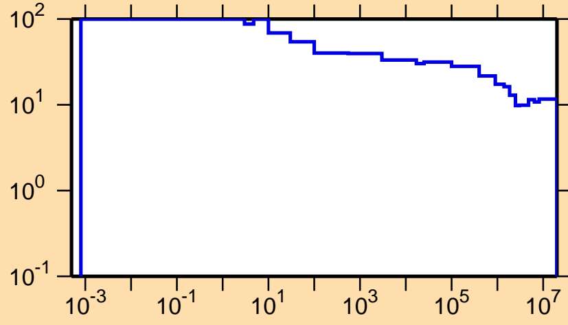
\Delta\sigma/\sigma vs. E for ^{140}\text{Gd}(n,\text{nonel.})
