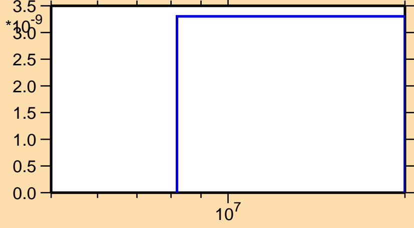
\sigma vs. E for ^{140}\text{Gd}(n,\text{pt})
