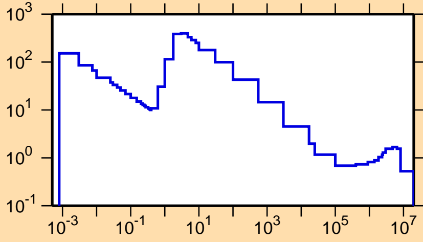
\sigma vs. E for ^{140}\text{Gd}(n,p)
