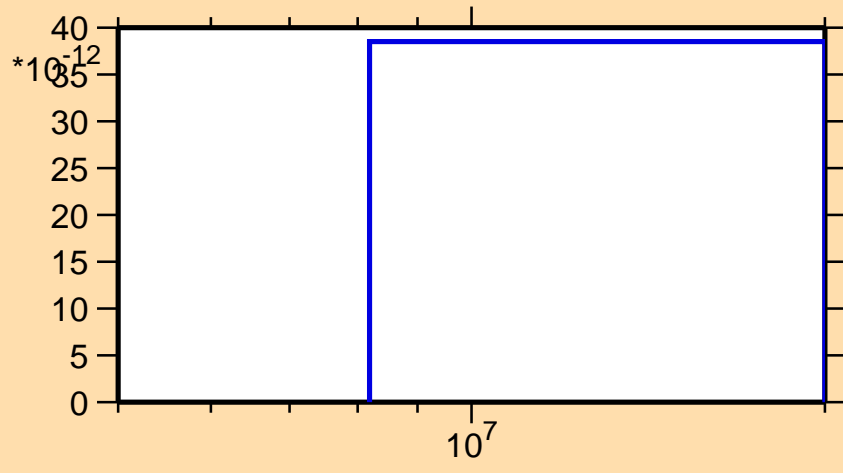
\sigma vs. E for ^{140}\text{Gd}(n,2n\alpha)
