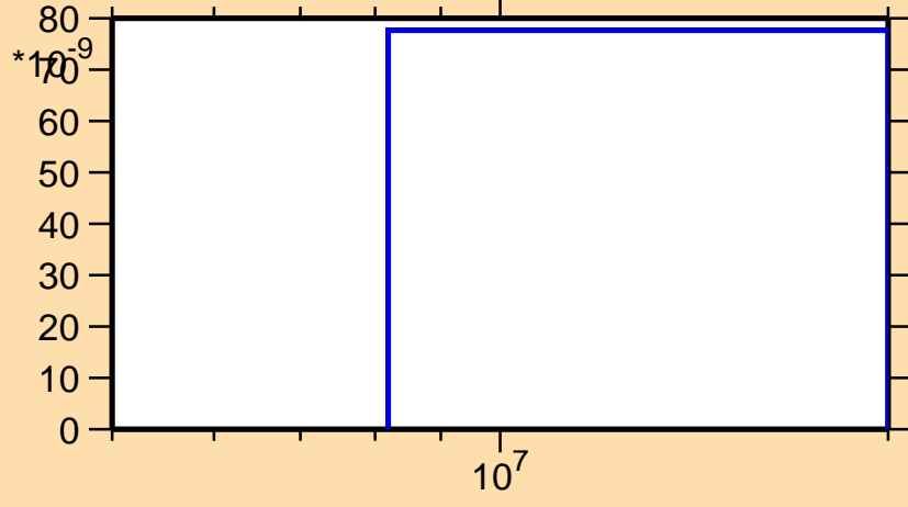
\sigma vs. E for ^{140}\text{Gd}(\text{mt } 45)
