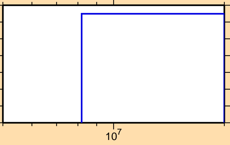
\sigma vs. E for ^{140}\text{Gd}(n,2np)
