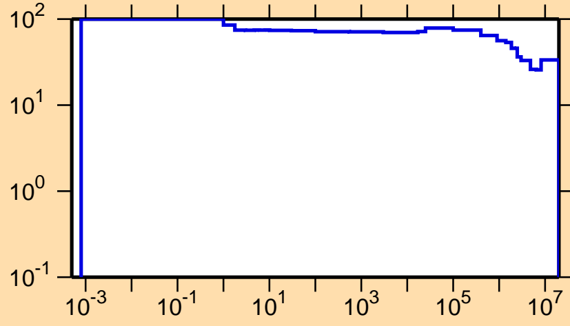
\Delta\sigma/\sigma vs. E for ^{140}\text{Gd}(n,p)
