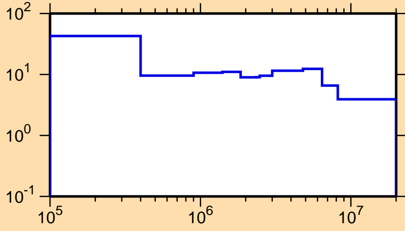
\Delta\sigma/\sigma vs. E for ^{140}\text{Gd}(n,\text{tot.})
