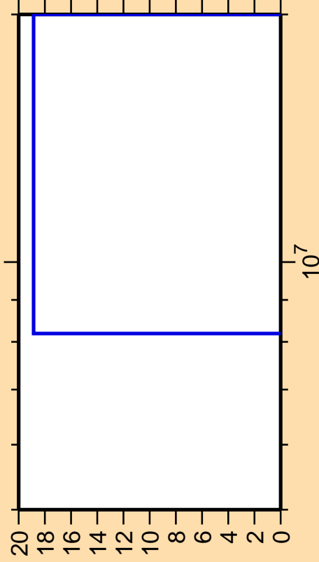
\Delta\sigma/\sigma vs. E for ^{140}\text{Gd} (mt 34)
