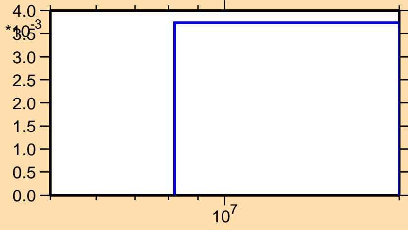
\sigma vs. E for ^{140}\text{Gd}(n,2n)
