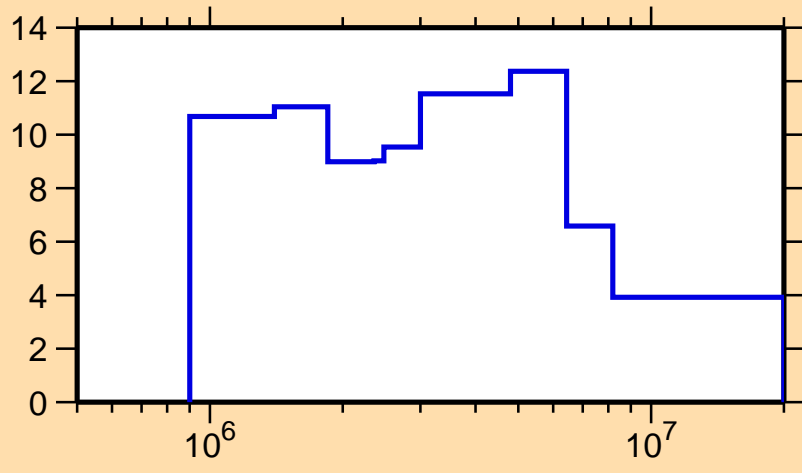
\Delta\sigma/\sigma vs. E for ^{140}\text{Gd}(n,\text{tot.})
