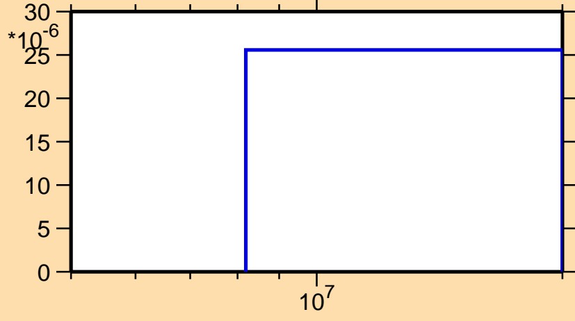
\sigma vs. E for ^{140}\text{Gd}(n,t)
