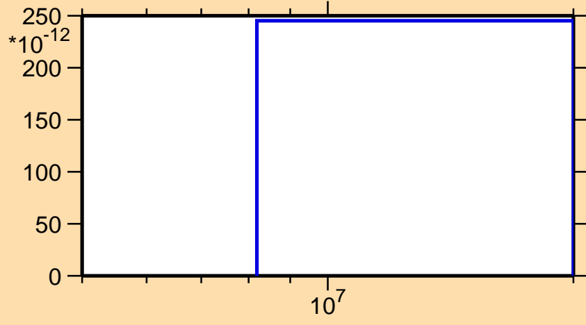
\sigma vs. E for ^{140}\text{Gd}(\text{mt117})
