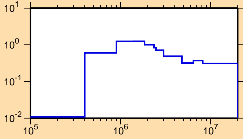
\sigma vs. E for ^{140}\text{Gd}(n,\text{inel.})
