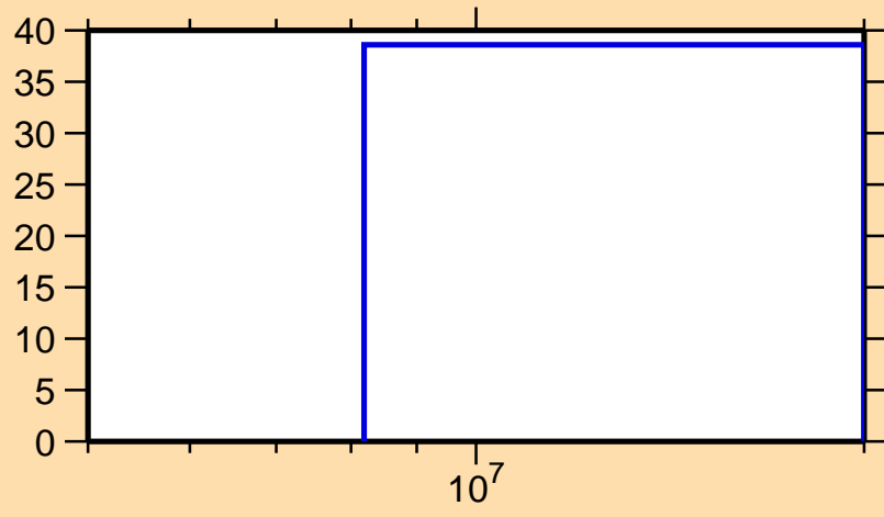
\Delta\sigma/\sigma vs. E for ^{140}\text{Gd}(n,\text{inel.})
