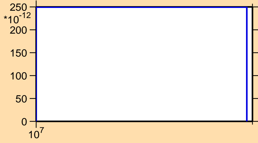
\sigma vs. E for ^{141}\text{Gd} (mt 34)
