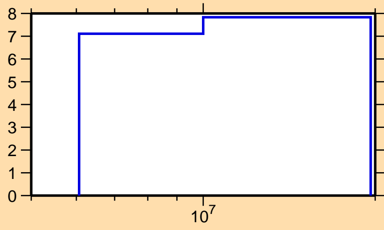
\Delta\sigma/\sigma vs. E for ^{141}\text{Gd}(n,\text{nonel.})
