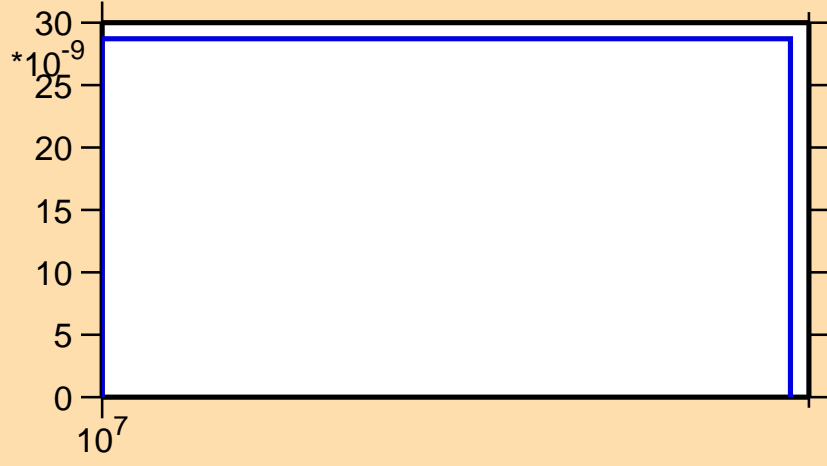
\sigma vs. E for ^{141}\text{Gd}(n,2n\alpha)
