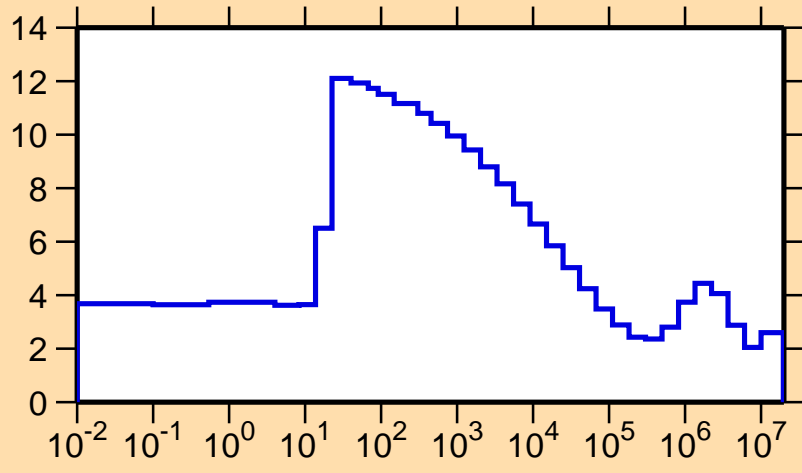
\sigma vs. E for ^{141}\text{Gd}(n,\text{el.})
