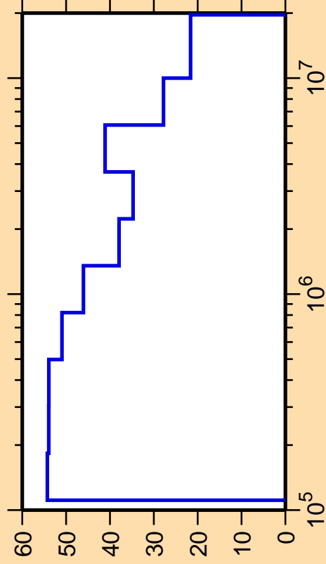
\Delta\sigma/\sigma vs. E for ^{141}\text{Gd}(n,\text{inel.})
