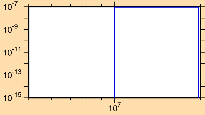
\sigma vs. E for ^{141}\text{Gd}(\text{mt } 45)
