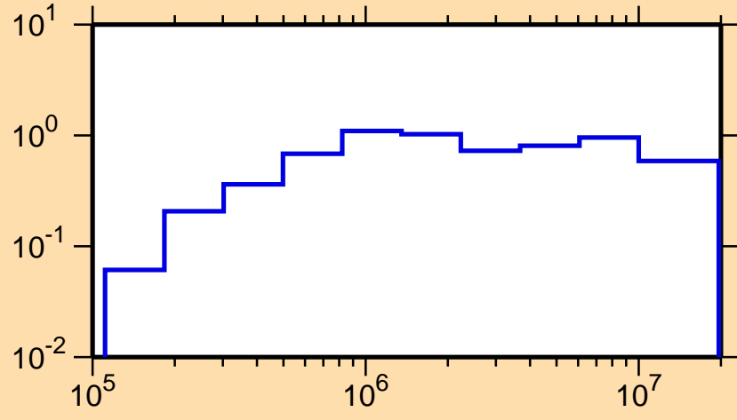
\sigma vs. E for ^{141}\text{Gd}(n,\text{inel.})
