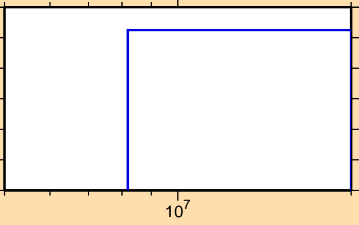
\sigma vs. E for ^{141}\text{Gd}(n,2n)
