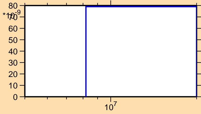
\sigma vs. E for ^{141}\text{Gd} (mt 45)
