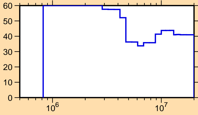
\Delta\sigma/\sigma vs. E for ^{141}\text{Gd}(n,n\text{cont.})
