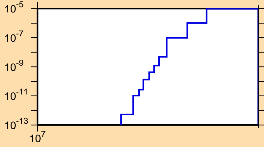
\sigma vs. E for ^{141}\text{Gd}(n,\text{nd})
