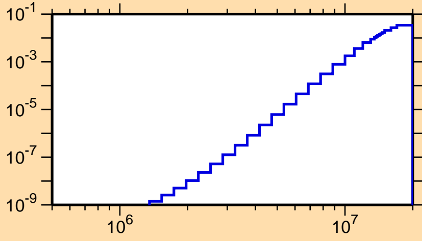
\sigma vs. E for ^{141}\text{Gd}(n,p\alpha)
