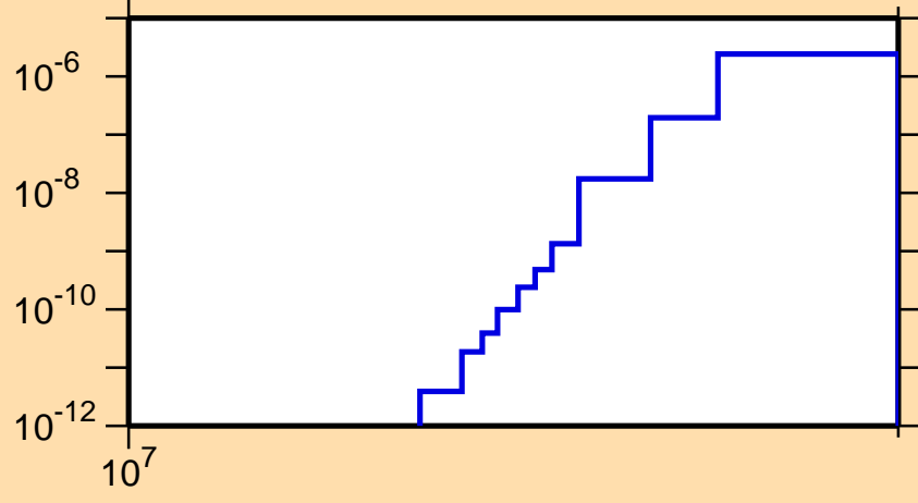
\sigma vs. E for ^{141}\text{Gd}(n,2n\alpha)
