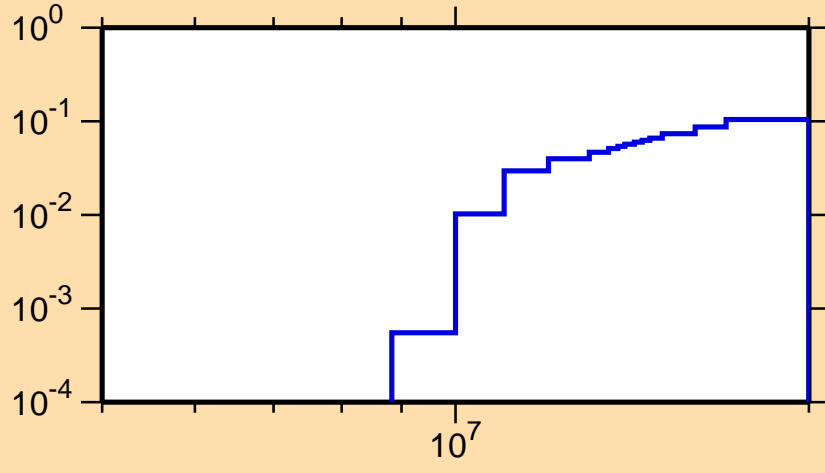
\sigma vs. E for ^{141}\text{Gd}(n,2n)
