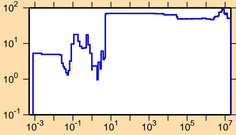
\Delta\sigma/\sigma vs. E for ^{141}\text{Gd}(n,\gamma)
