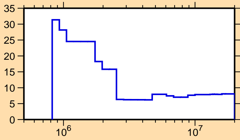
\Delta\sigma/\sigma vs. E for ^{141}\text{Gd}(n,\text{nonel.})
