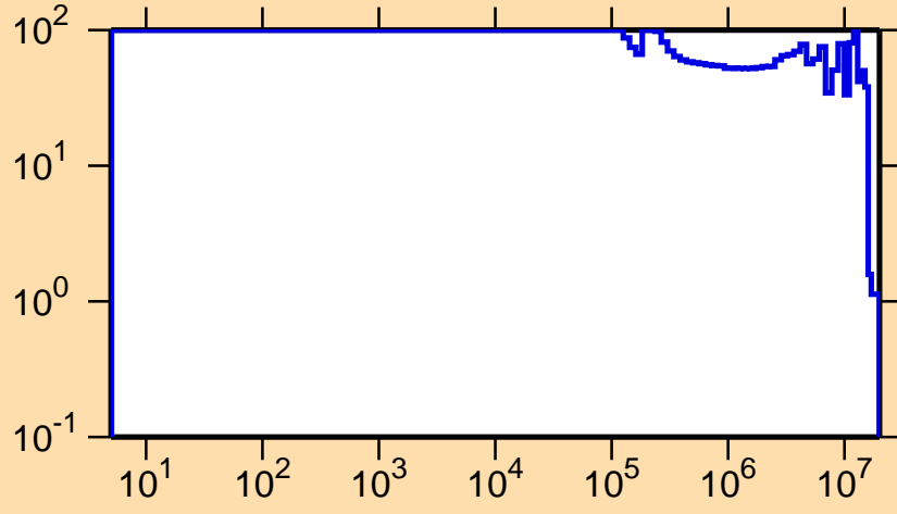
\Delta\sigma/\sigma vs. E for ^{141}\text{Gd}(n,n_1)
