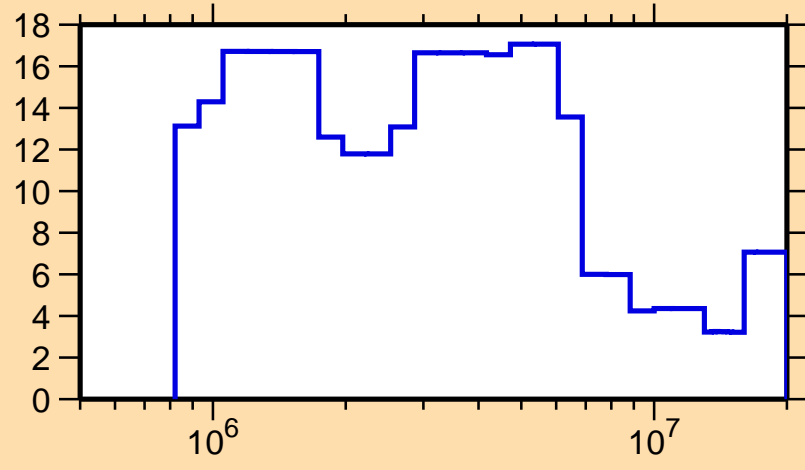
\Delta\sigma/\sigma vs. E for ^{141}\text{Gd}(n,\text{tot.})
