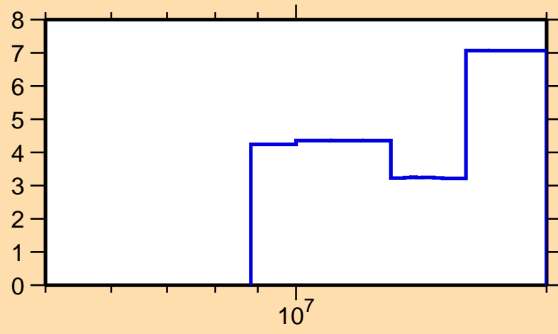
\Delta\sigma/\sigma vs. E for ^{141}\text{Gd}(n,\text{tot.})
