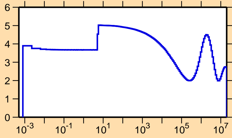
\sigma vs. E for ^{141}\text{Gd}(n,\text{el.})
