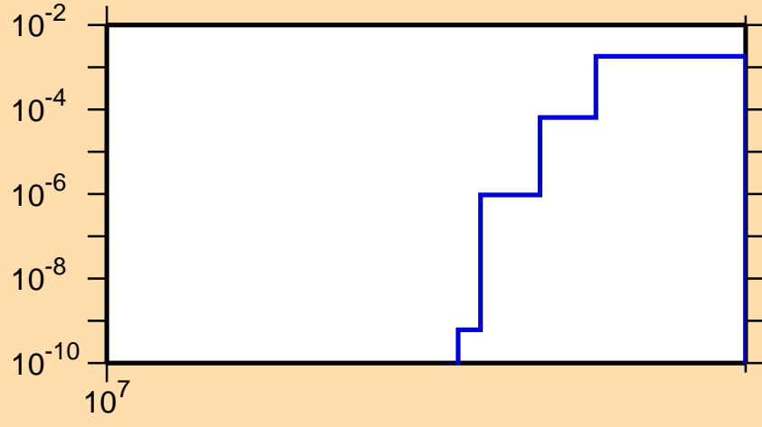
\sigma vs. E for ^{141}\text{Gd}(n,2np)
