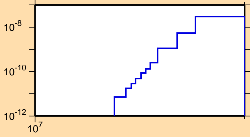
\sigma vs. E for ^{141}\text{Gd}(\text{mt117})
