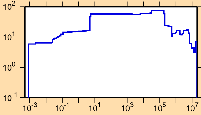
\Delta\sigma/\sigma vs. E for ^{141}\text{Gd}(n,\text{tot.})
