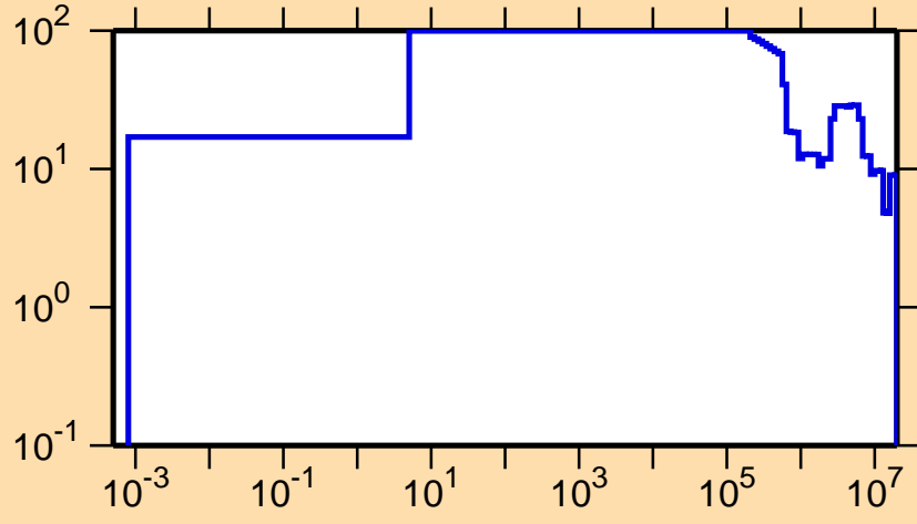
\Delta\sigma/\sigma vs. E for ^{141}\text{Gd}(n,\text{el.})
