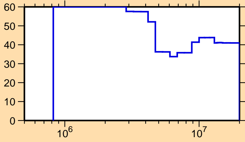
\Delta\sigma/\sigma vs. E for ^{141}\text{Gd}(n,n\text{cont.})
