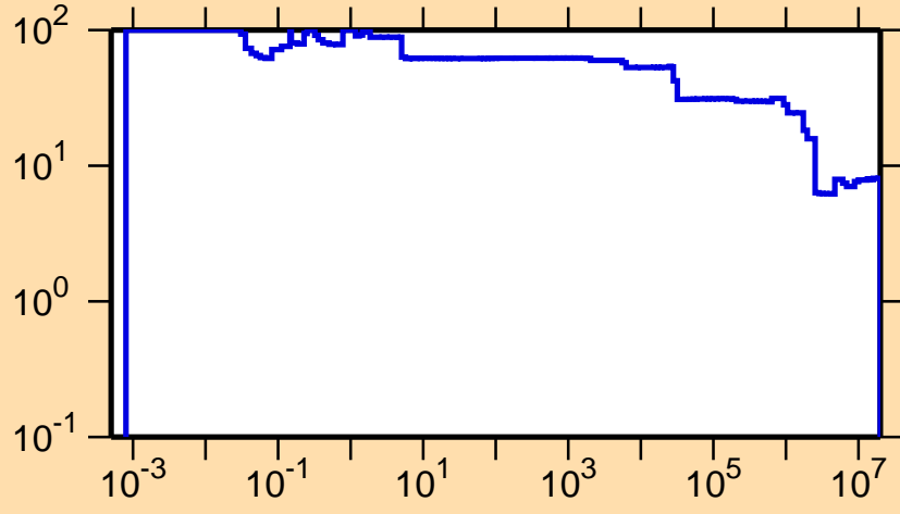
\Delta\sigma/\sigma vs. E for ^{141}\text{Gd}(n,\text{nonel.})
