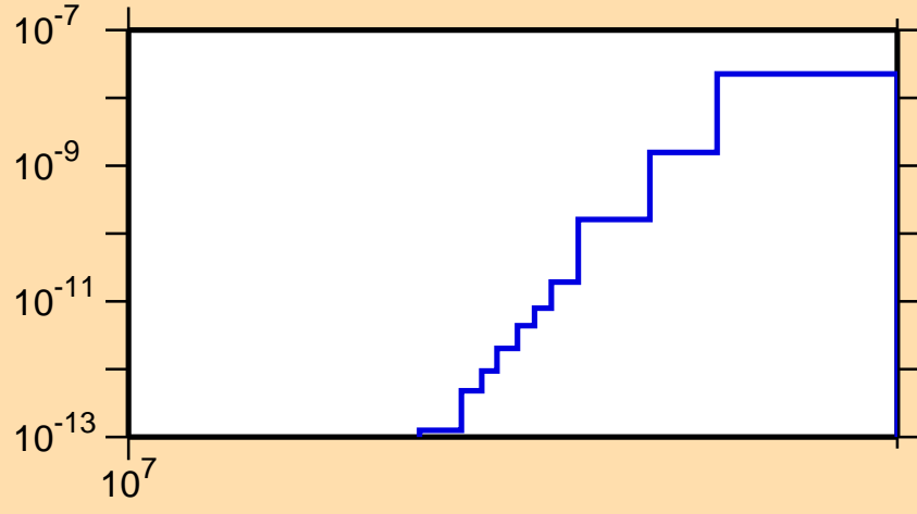
\sigma vs. E for ^{141}\text{Gd}(\text{mt } 34)
