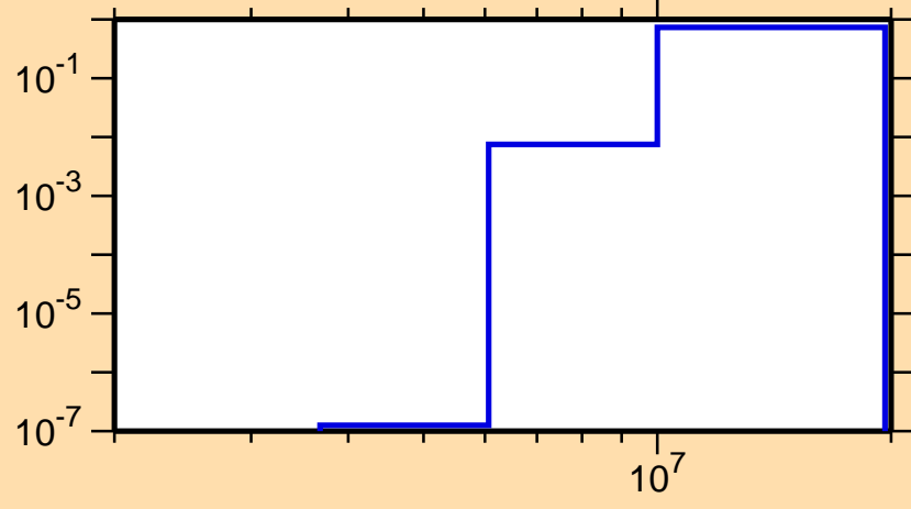
\sigma vs. E for ^{141}\text{Gd}(n,np)
