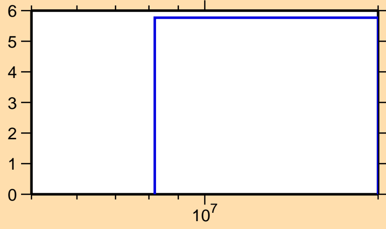
\Delta\sigma/\sigma vs. E for ^{141}\text{Gd}(n,\text{el.})
