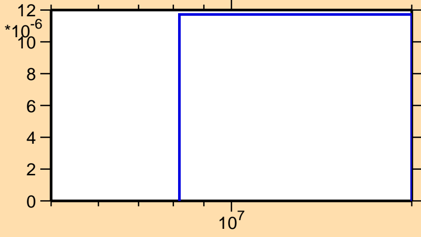
\sigma vs. E for ^{141}\text{Gd}(n,\text{pd})
