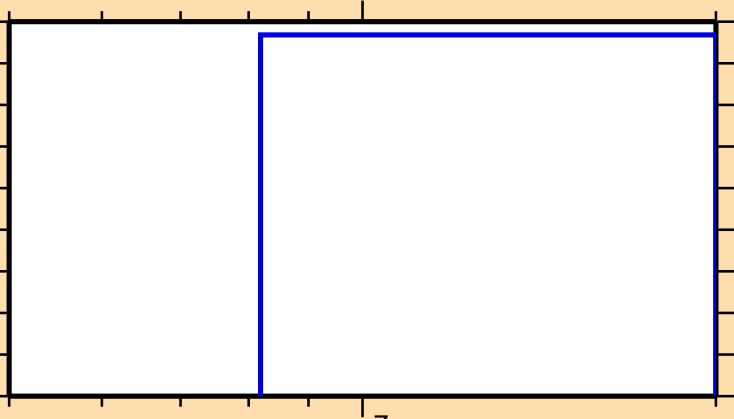
\sigma vs. E for ^{141}\text{Gd}(n,2np)
