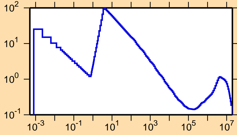
\sigma vs. E for ^{142}\text{Gd}(n,p)
