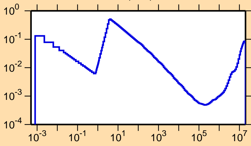
\sigma vs. E for ^{142}\text{Gd}(n,\alpha)
