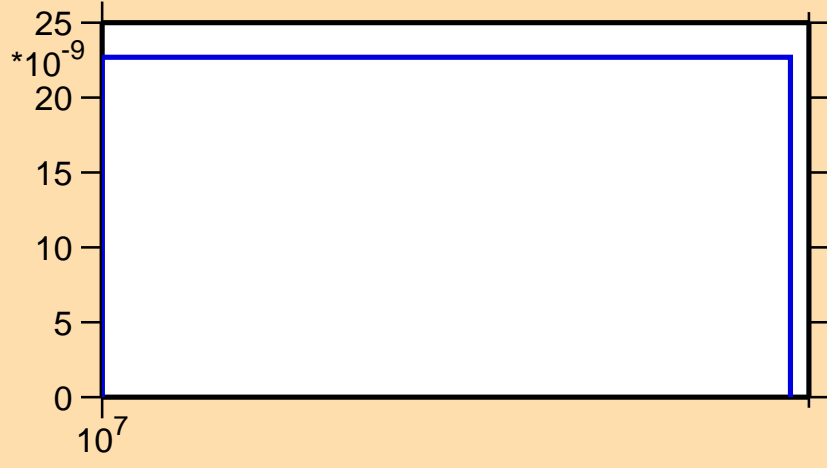
\sigma vs. E for ^{142}\text{Gd} (mt 45)
