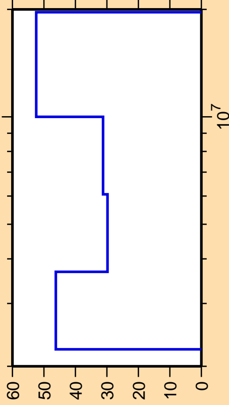
\Delta\sigma/\sigma vs. E for ^{142}\text{Gd}(n,n\text{cont.})
