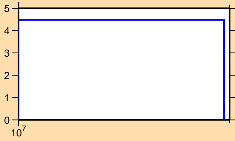
\Delta\sigma/\sigma vs. E for ^{142}\text{Gd}(n,\text{el.})
