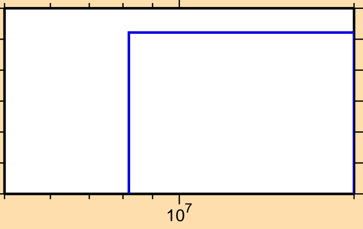
\sigma vs. E for ^{143}\text{Gd}(n,2n\alpha)
