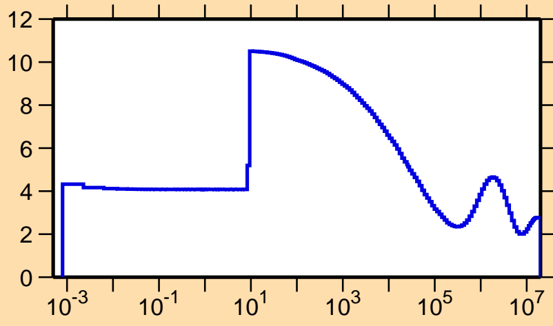
\sigma vs. E for ^{143}\text{Gd}(n,\text{el.})
