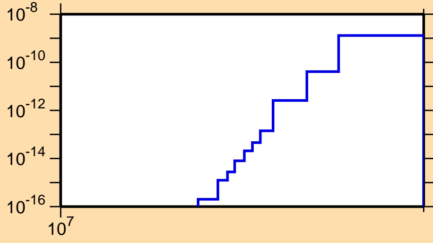
\sigma vs. E for ^{143}\text{Gd} (mt 34)
