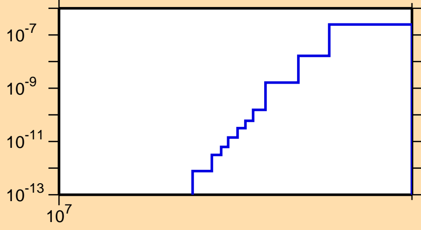
\sigma vs. E for ^{143}\text{Gd} (mt 45)
