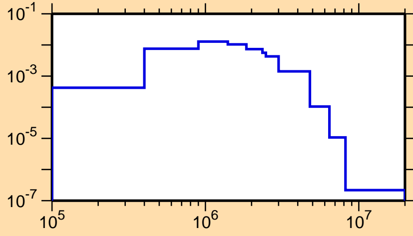
\sigma vs. E for ^{143}\text{Gd}(n,n_3)
