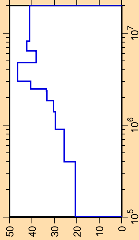
\Delta\sigma/\sigma vs. E for ^{143}\text{Gd}(n,n_3)
