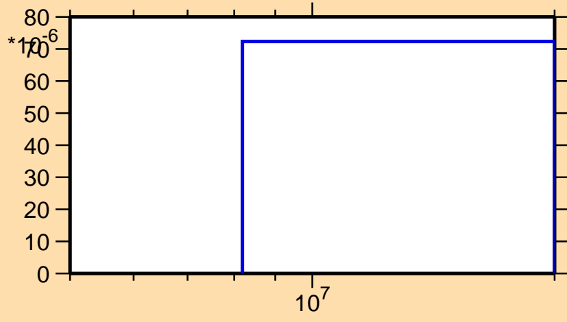
\sigma vs. E for ^{143}\text{Gd}(n,t)
