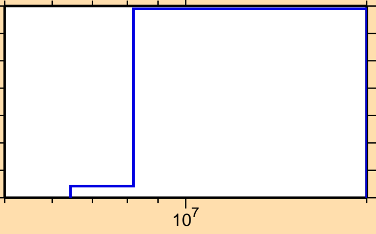
\sigma vs. E for ^{143}\text{Gd}(n,\text{He3})
