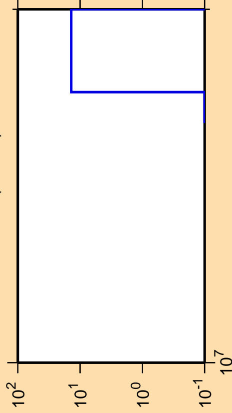
\Delta\sigma/\sigma vs. E for ^{144}\text{Gd} (mt 34)
