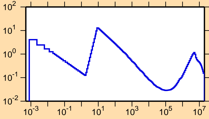
\sigma vs. E for ^{144}\text{Gd}(n,p)
