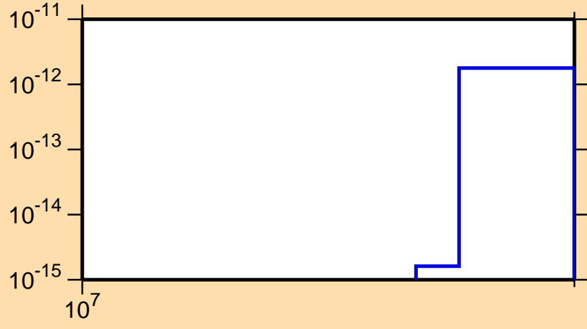
\sigma vs. E for ^{144}\text{Gd} (mt 34)
