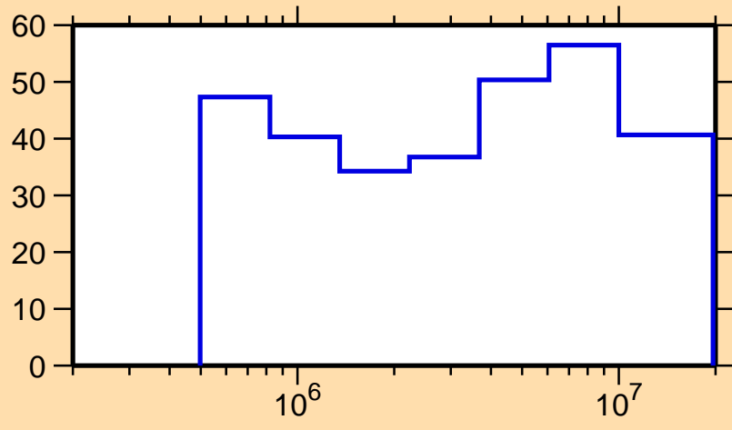
\Delta\sigma/\sigma vs. E for ^{144}\text{Gd}(n,n_1)
