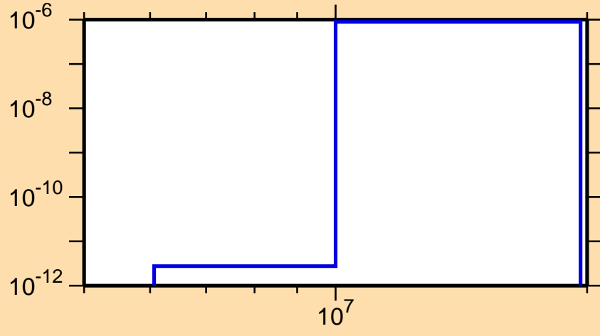
\sigma vs. E for ^{144}\text{Gd}(n,\text{He3})
