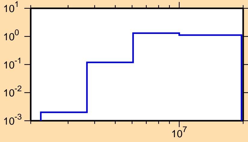
\sigma vs. E for ^{144}\text{Gd}(n,n\text{cont.})
