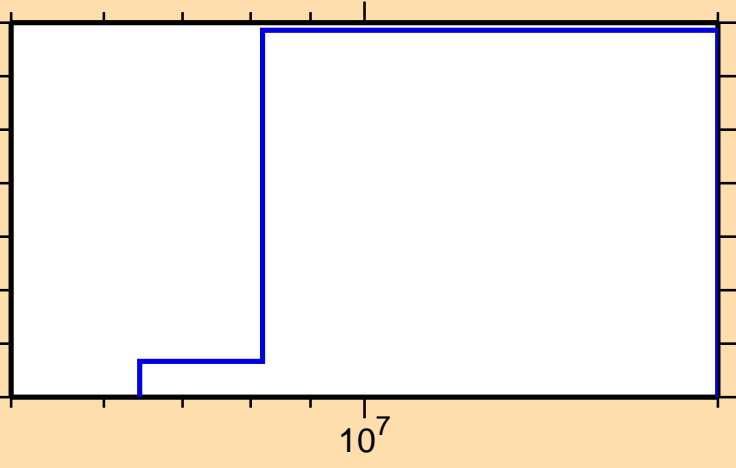
\sigma vs. E for ^{144}\text{Gd}(n,\text{He3})
