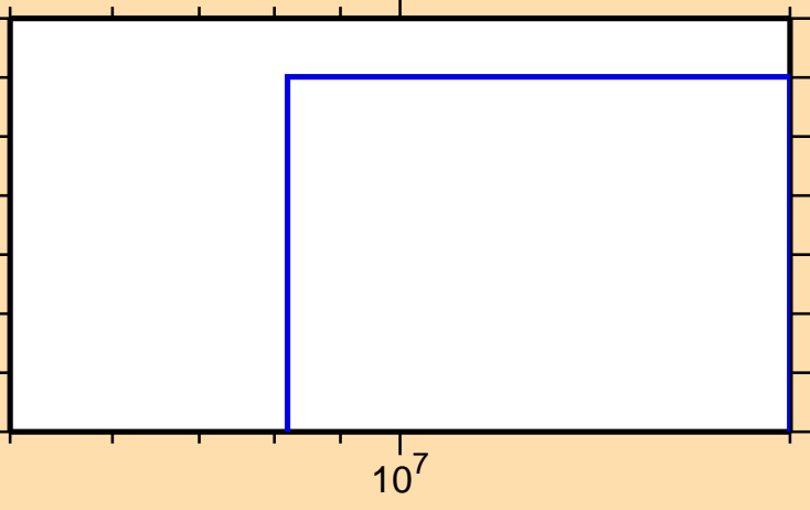
\sigma vs. E for ^{144}\text{Gd}(n,t)
