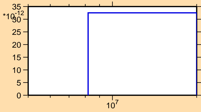
\sigma vs. E for ^{144}\text{Gd}(n,2n\alpha)
