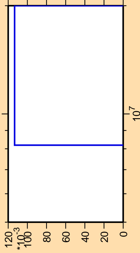
\Delta\sigma/\sigma vs. E for ^{144}\text{Gd}(\text{mt } 34)
