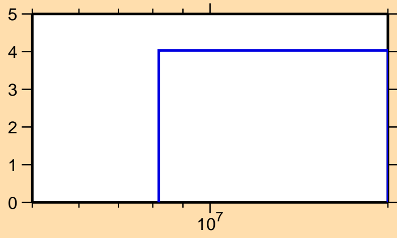
\Delta\sigma/\sigma vs. E for ^{144}\text{Gd}(n,\text{tot.})
