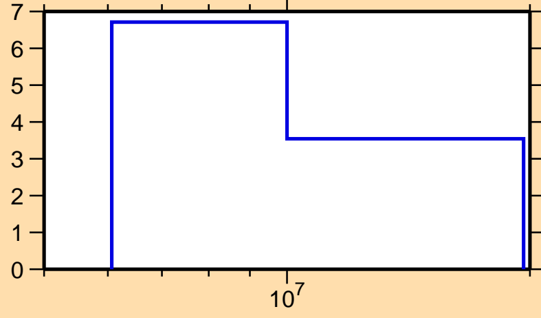
\Delta\sigma/\sigma vs. E for ^{145}\text{Gd}(n,\text{el.})
