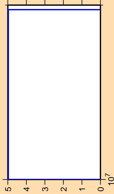
\Delta\sigma/\sigma vs. E for ^{145}\text{Gd} (mt 34)
