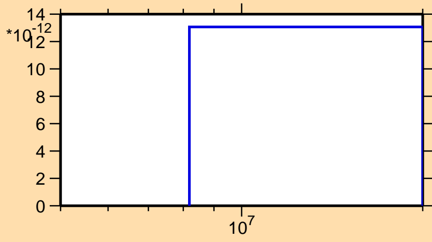
\sigma vs. E for ^{145}\text{Gd}(\text{mt } 45)
