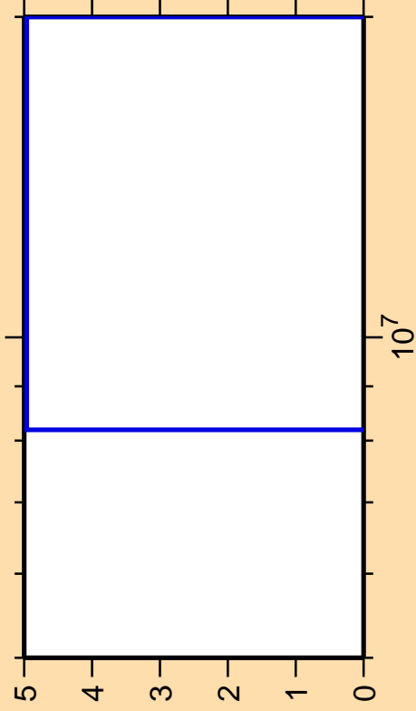
\Delta\sigma/\sigma vs. E for ^{145}\text{Gd}(\text{mt } 34)
