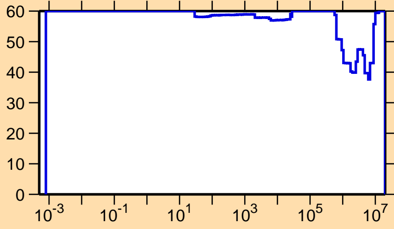
\Delta\sigma/\sigma vs. E for ^{145}\text{Gd}(n,p)
