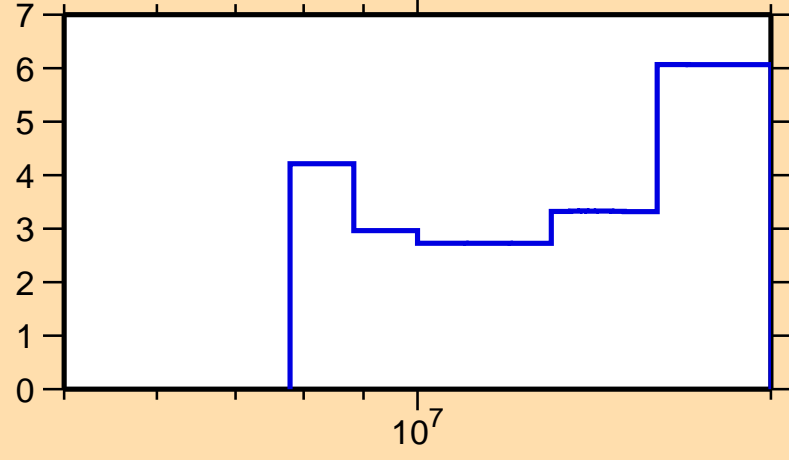
\Delta\sigma/\sigma vs. E for ^{145}\text{Gd}(n,\text{tot.})
