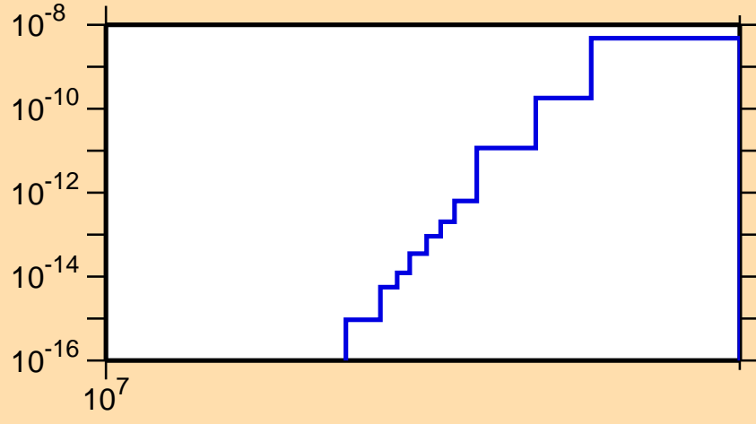
\sigma vs. E for ^{145}\text{Gd} (mt 45)
