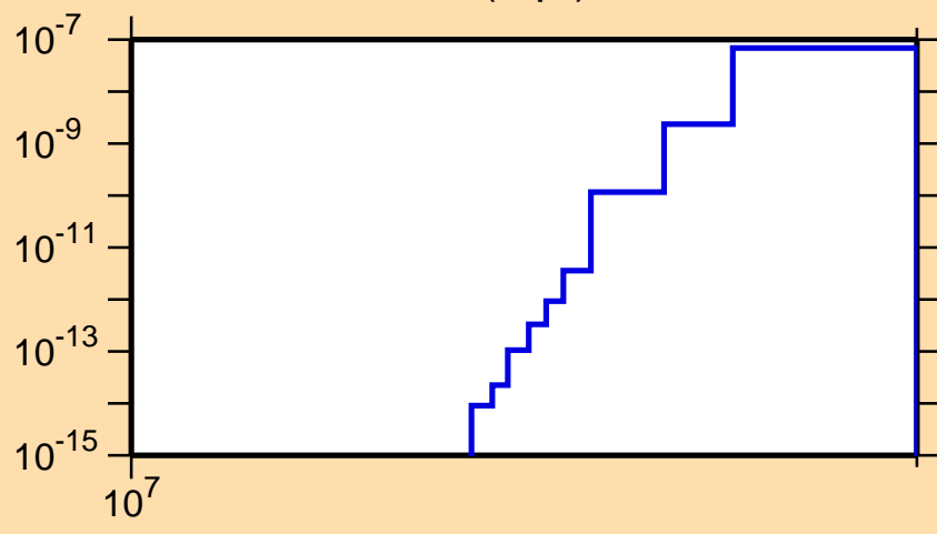
\sigma vs. E for ^{145}\text{Gd}(n,\text{pt})
