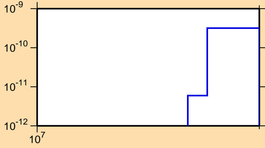
\sigma vs. E for ^{145}\text{Gd} (mt 34)
