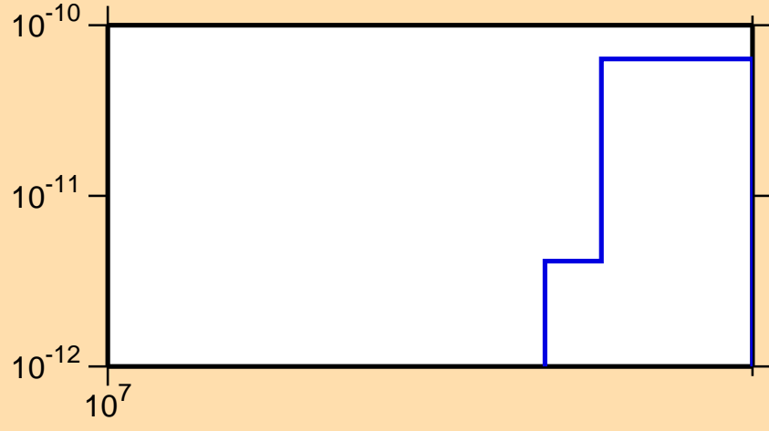
\sigma vs. E for ^{145}\text{Gd}(\text{mt117})
