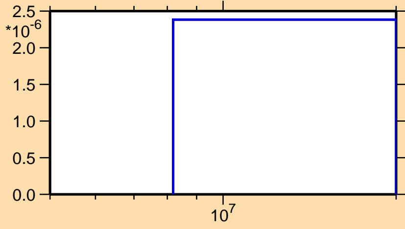
\sigma vs. E for ^{145}\text{Gd}(n,2np)
