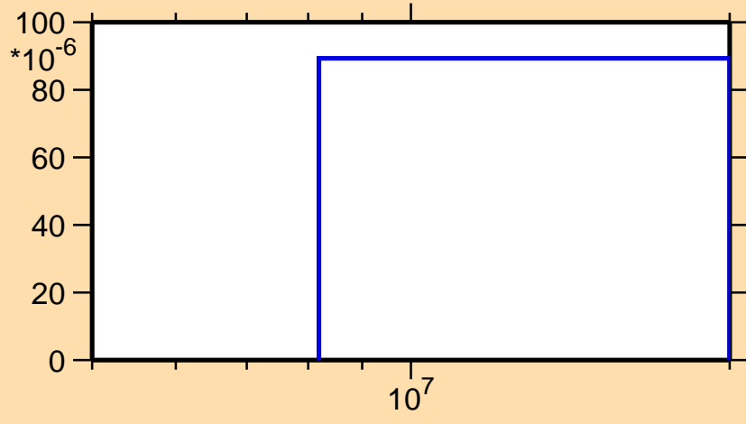
\sigma vs. E for ^{145}\text{Gd}(n,t)
