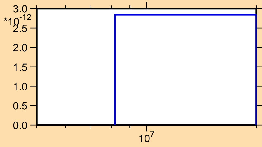
\sigma vs. E for ^{145}\text{Gd}(\text{mt } 34)
