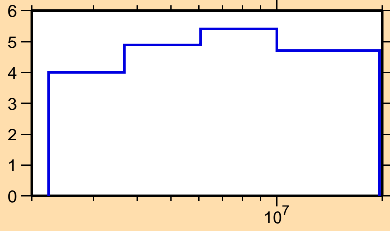
\Delta\sigma/\sigma vs. E for ^{146}\text{Gd}(n,n\text{onel.})
