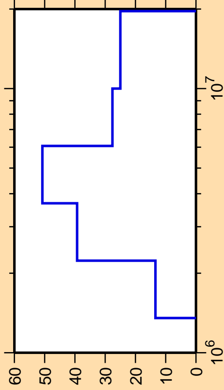
\Delta\sigma/\sigma vs. E for ^{146}\text{Gd}(n,n_1)
