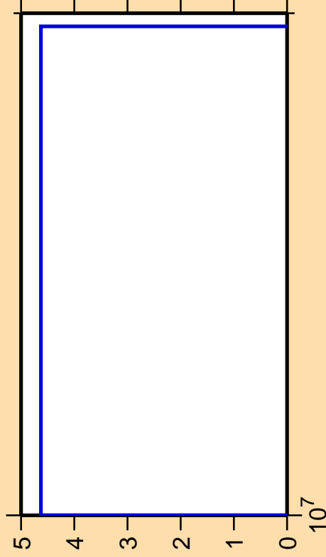
\Delta\sigma/\sigma vs. E for ^{146}\text{Gd} (mt 45)
