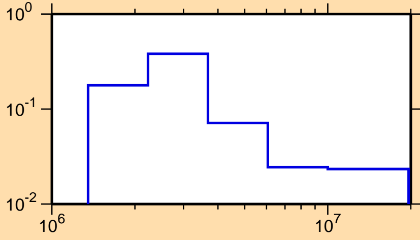
\sigma vs. E for ^{146}\text{Gd}(n,n_1)
