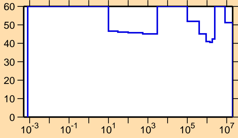
\Delta\sigma/\sigma vs. E for ^{146}\text{Gd}(n,p)
