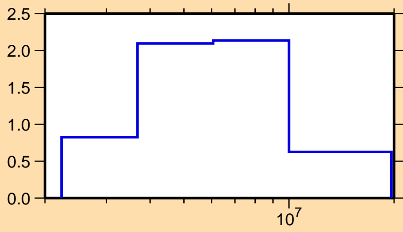
\sigma vs. E for ^{147}\text{Gd}(n,n\text{cont.})
