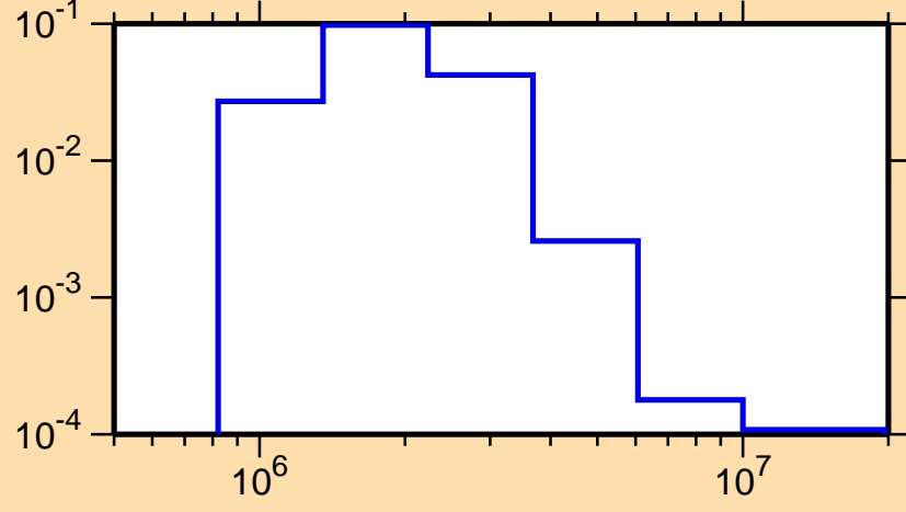
\sigma vs. E for ^{147}\text{Gd}(n,n_1)
