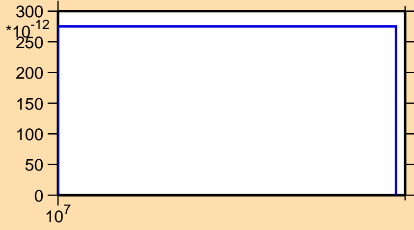
\sigma vs. E for ^{147}\text{Gd}(n,\text{pd})
