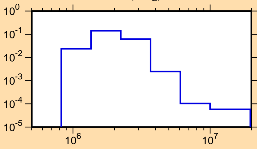
\sigma vs. E for ^{147}\text{Gd}(n,n_2)
