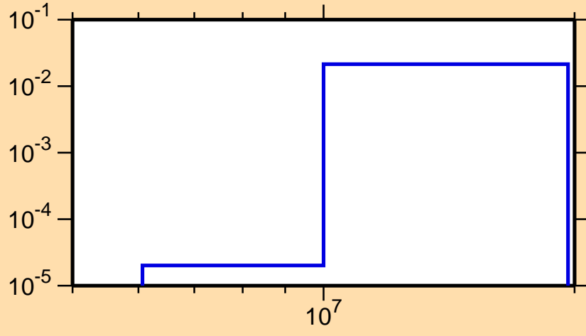
\sigma vs. E for ^{147}\text{Gd}(n,np)
