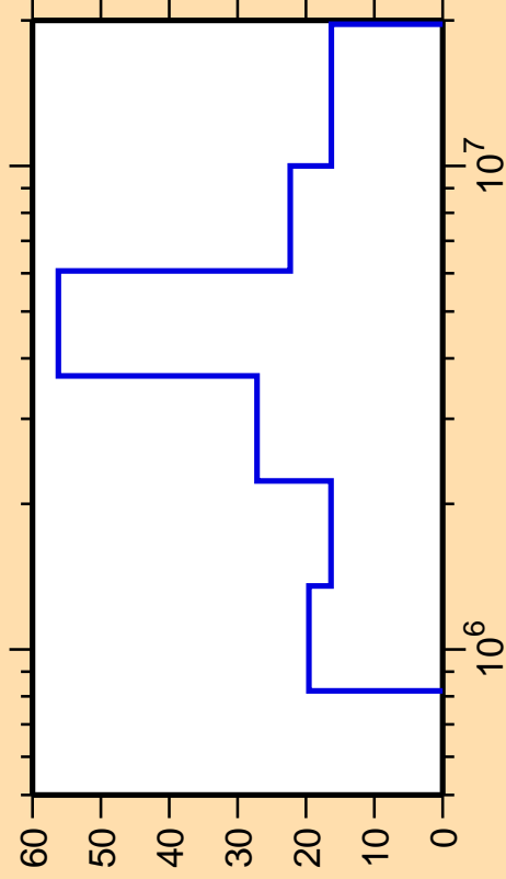
\Delta\sigma/\sigma vs. E for ^{147}\text{Gd}(n,n_2)
