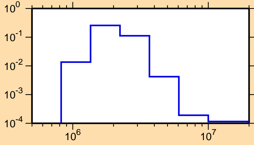
\sigma vs. E for ^{147}\text{Gd}(n,n_3)
