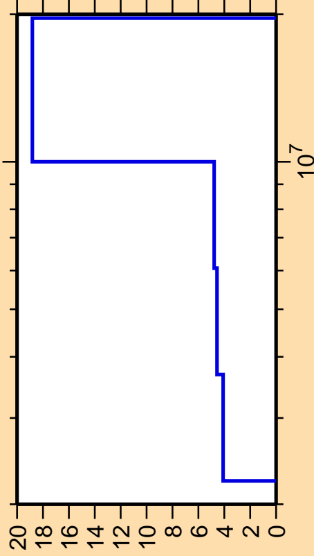
\Delta\sigma/\sigma vs. E for ^{147}\text{Gd}(n,n\text{cont.})
