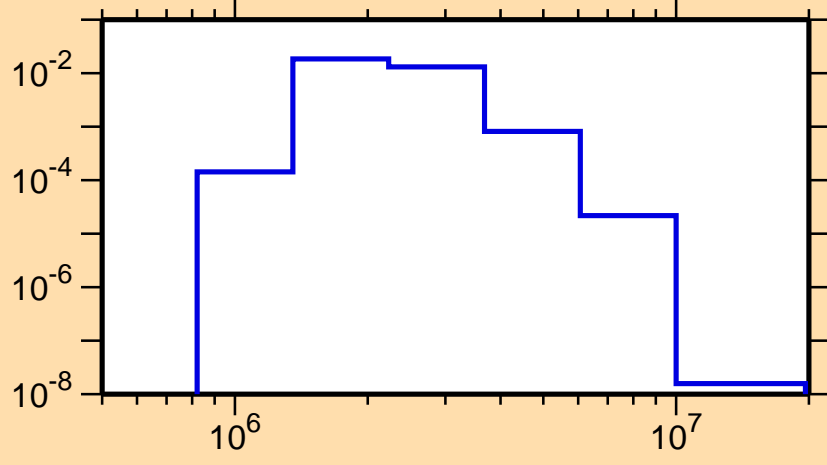
\sigma vs. E for ^{147}\text{Gd}(n,n_4)
