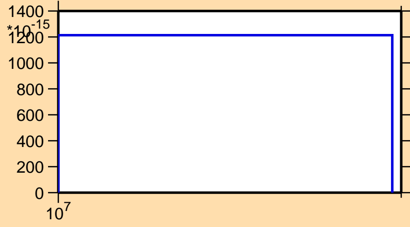
\sigma vs. E for ^{147}\text{Gd}(\text{mt117})
