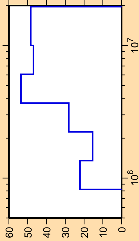
\Delta\sigma/\sigma vs. E for ^{147}\text{Gd}(n,n_4)
