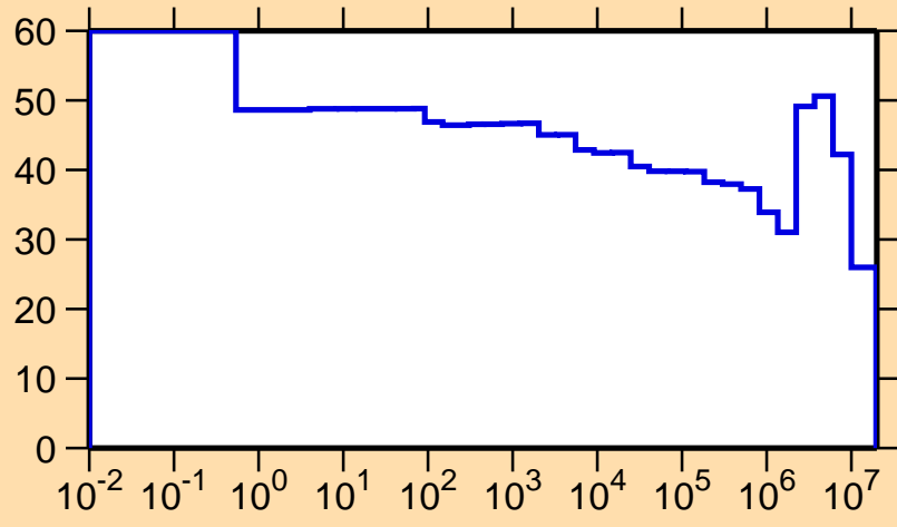
\Delta\sigma/\sigma vs. E for ^{147}\text{Gd}(n,p)
