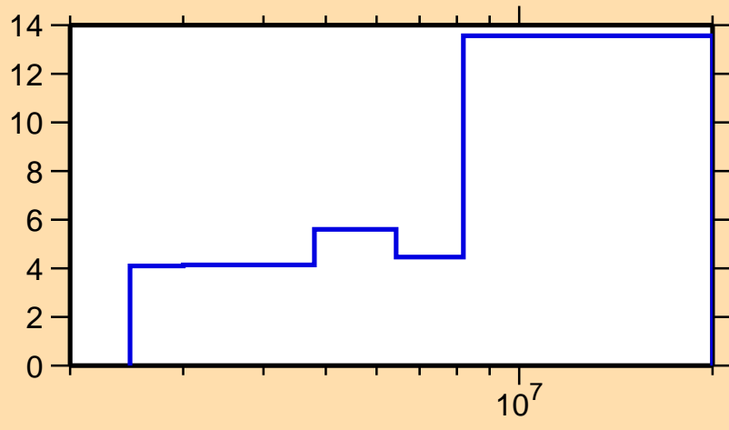
\Delta\sigma/\sigma vs. E for ^{147}\text{Gd}(n,n\text{cont.})
