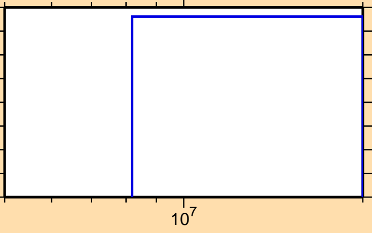
\sigma vs. E for ^{147}\text{Gd}(n,2np)
