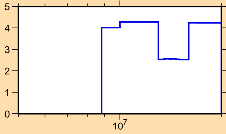
\Delta\sigma/\sigma vs. E for ^{148}\text{Gd}(n,\text{el.})
