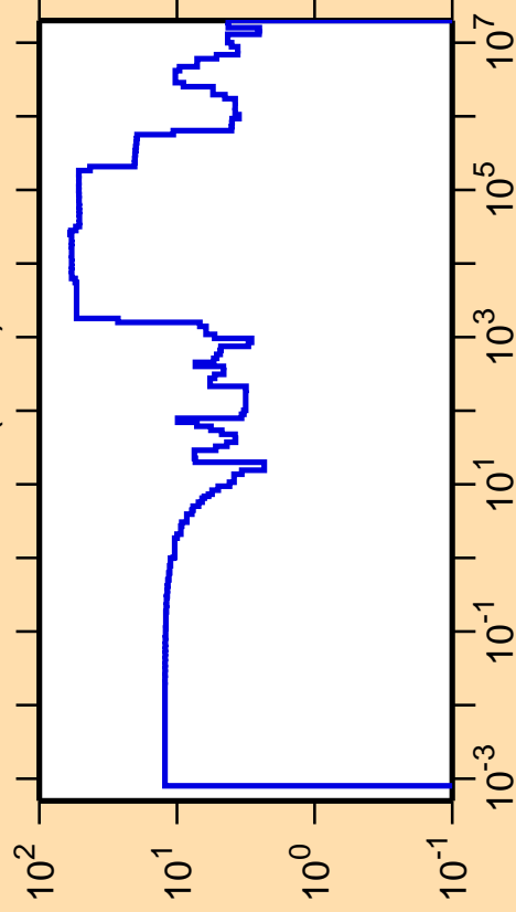
\Delta\sigma/\sigma vs. E for ^{148}\text{Gd}(n,\text{el.})
