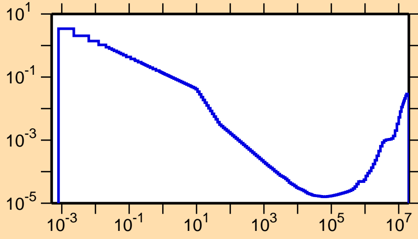
\sigma vs. E for ^{148}\text{Gd}(n,\alpha)
