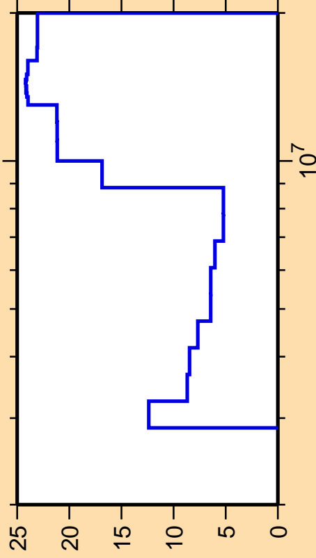
\Delta\sigma/\sigma vs. E for ^{148}\text{Gd}(n,n\text{cont.})
