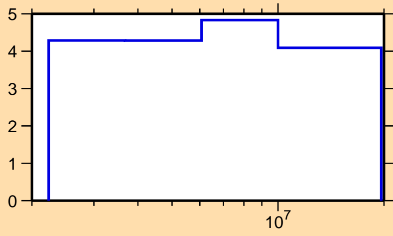
\Delta\sigma/\sigma vs. E for ^{148}\text{Gd}(n,n\text{onel.})
