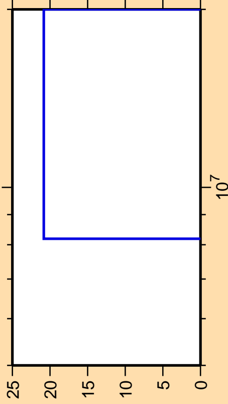
\Delta\sigma/\sigma vs. E for ^{148}\text{Gd}(n,n_1)
