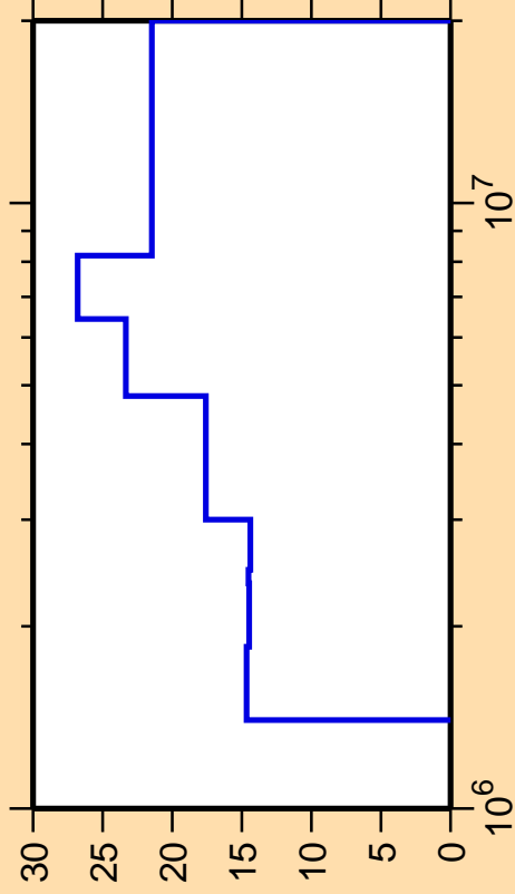
\Delta\sigma/\sigma vs. E for ^{148}\text{Gd}(n,n_3)
