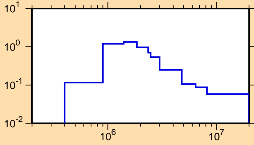
\sigma vs. E for ^{148}\text{Gd}(n,n_1)
