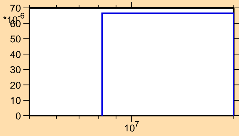
\sigma vs. E for ^{148}\text{Gd}(n,t)
