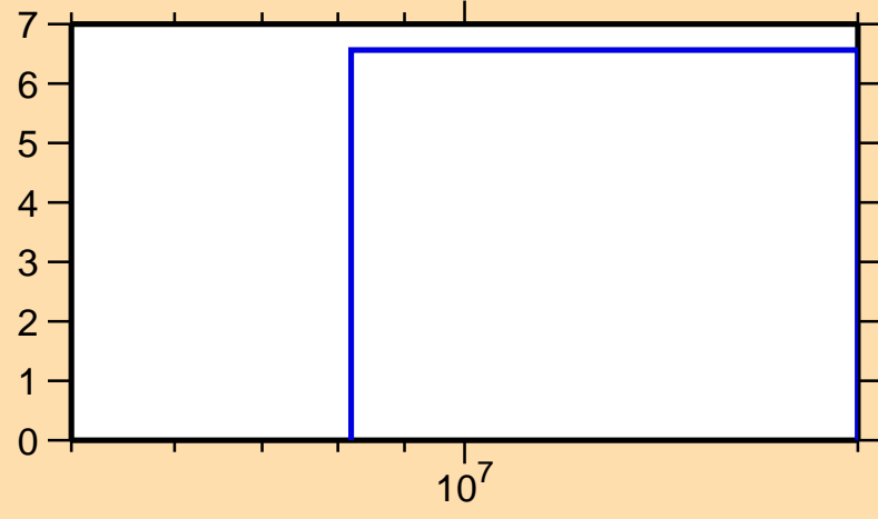
\Delta\sigma/\sigma vs. E for ^{148}\text{Gd}(n,2n)
