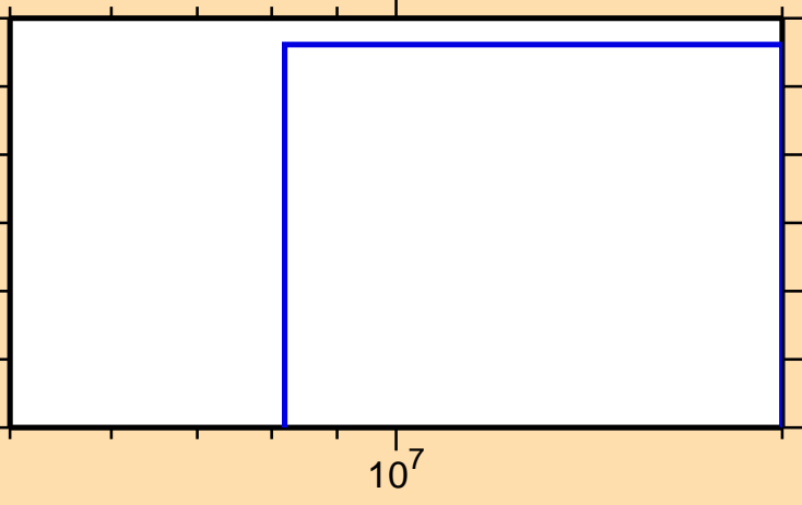
\sigma vs. E for ^{148}\text{Gd}(n,\text{nd})
