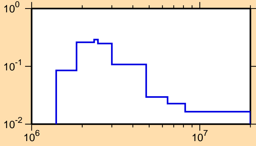
\sigma vs. E for ^{148}\text{Gd}(n,n_3)
