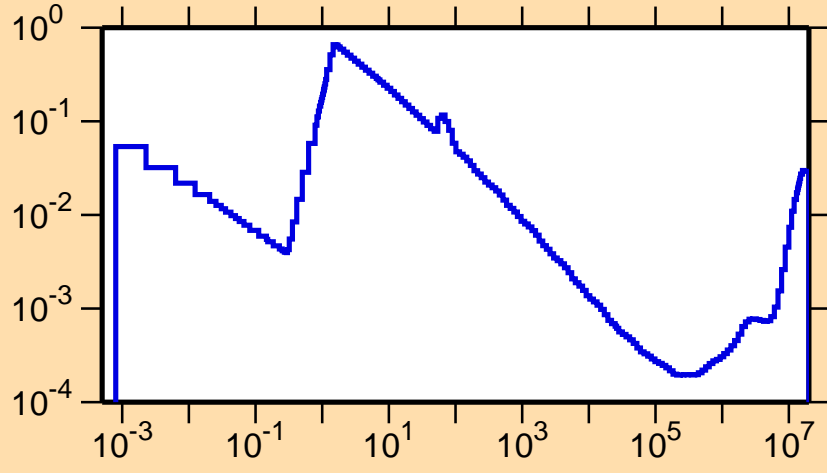
\sigma vs. E for ^{149}\text{Gd}(n,\alpha)
