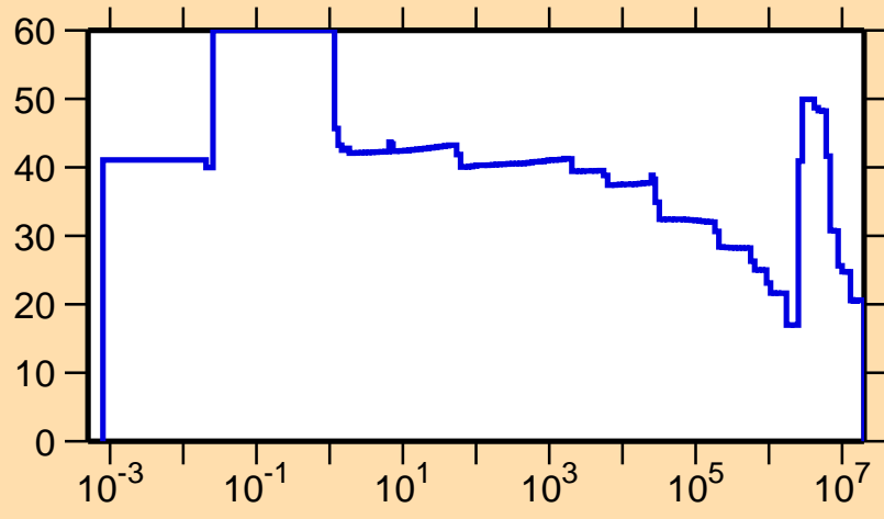
\Delta\sigma/\sigma vs. E for ^{149}\text{Gd}(n,p)
