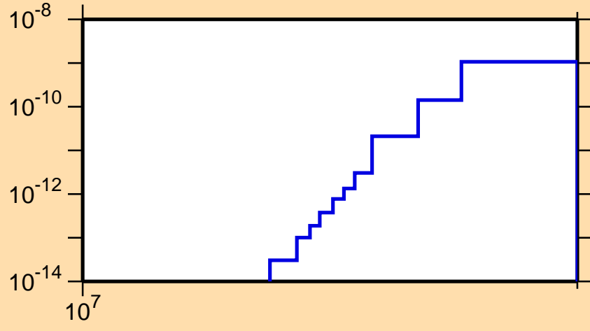
\sigma vs. E for ^{149}\text{Gd}(\text{mt117})
