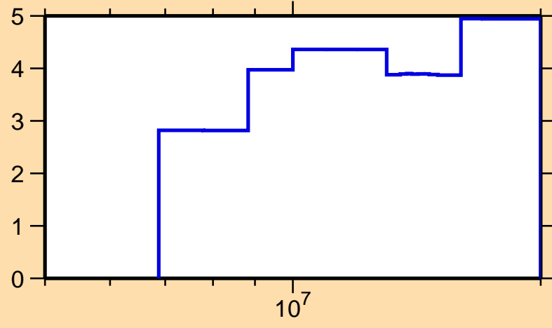
\Delta\sigma/\sigma vs. E for ^{149}\text{Gd}(n,\text{el.})
