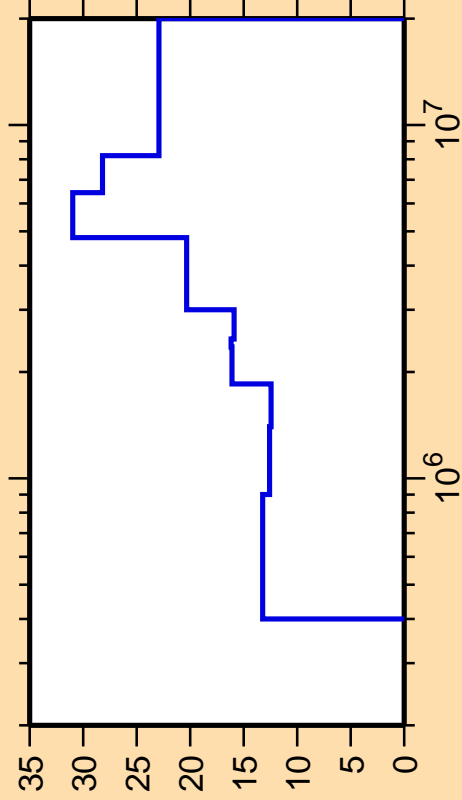
\Delta\sigma/\sigma vs. E for ^{149}\text{Gd}(n,n_4)
