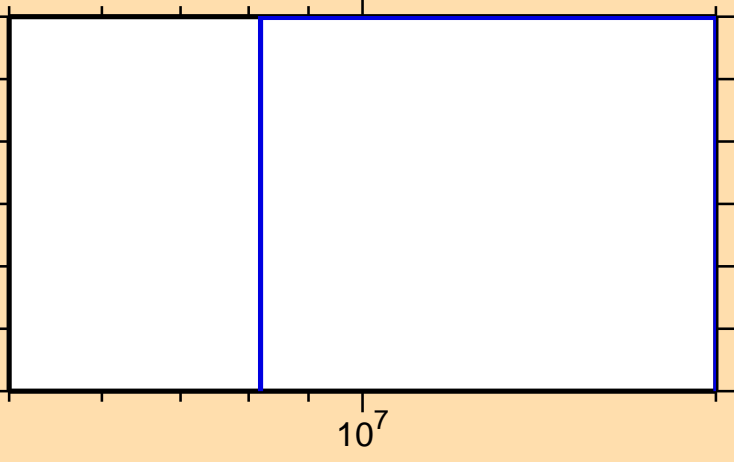
\sigma vs. E for ^{149}\text{Gd}(\text{mt } 11)
