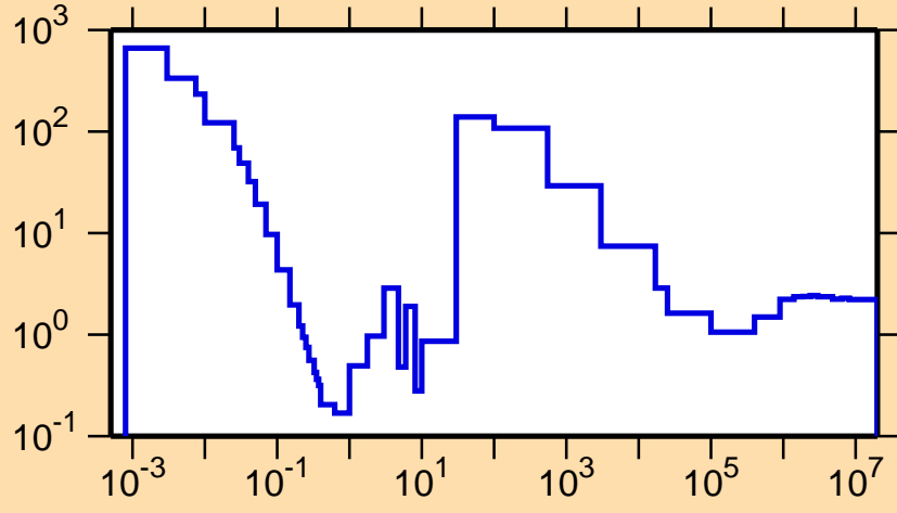
\sigma vs. E for ^{149}\text{Gd}(n,\text{nonel.})
