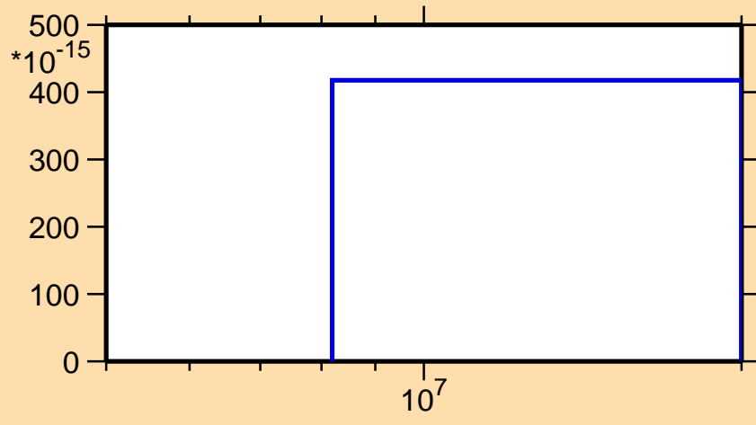
\sigma vs. E for ^{149}\text{Gd}(\text{mt } 34)
