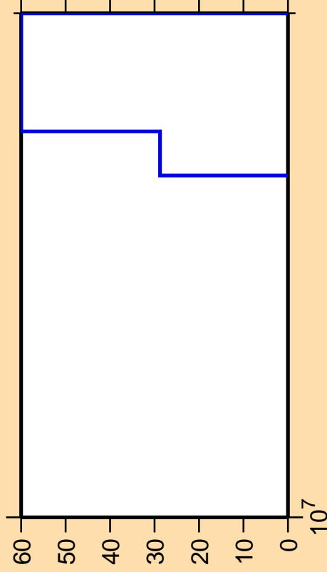
\Delta\sigma/\sigma vs. E for ^{150}\text{Gd} (mt 45)
