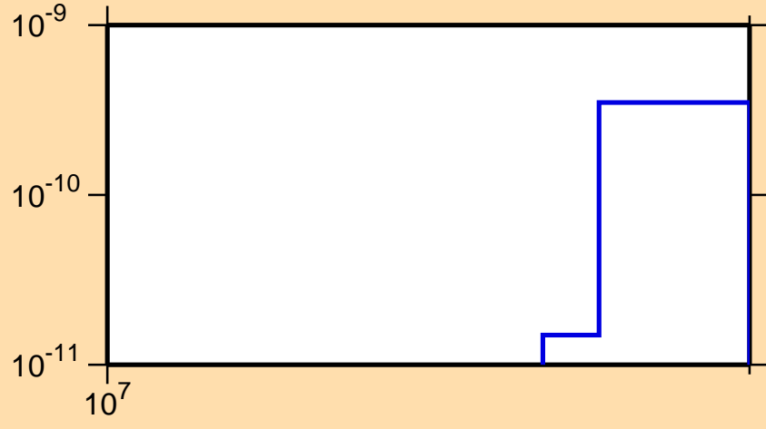
\sigma vs. E for ^{150}\text{Gd} (mt 45)
