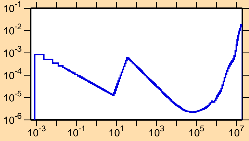
\sigma vs. E for ^{150}\text{Gd}(n,\alpha)
