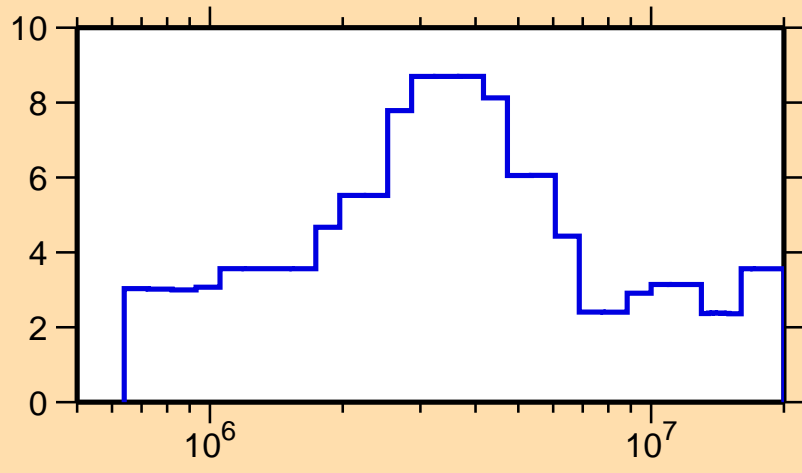
\Delta\sigma/\sigma vs. E for ^{150}\text{Gd}(n,\text{el.})
