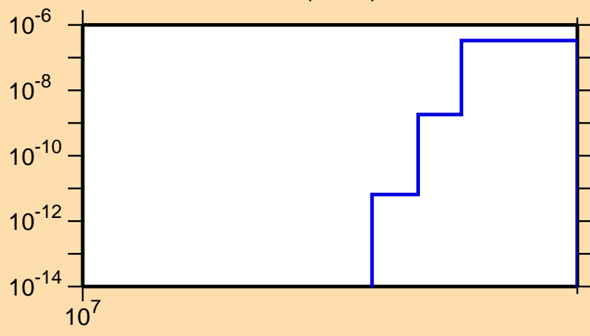
\sigma vs. E for ^{150}\text{Gd}(n,\text{nd})
