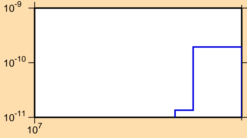
\sigma vs. E for ^{150}\text{Gd}(\text{mt117})
