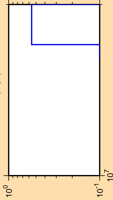
\Delta\sigma/\sigma vs. E for ^{150}\text{Gd}(n,\text{pt})
