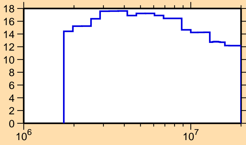
\Delta\sigma/\sigma vs. E for ^{150}\text{Gd}(n,n_1)
