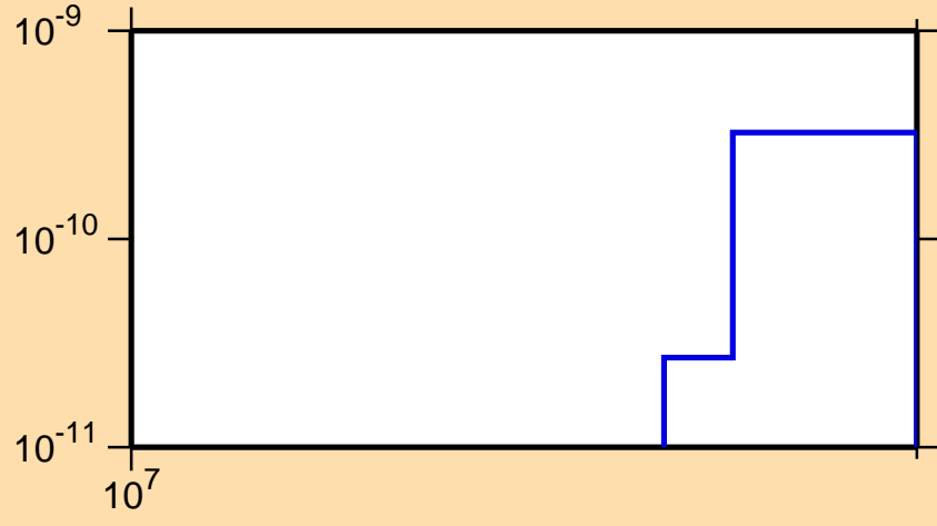
\sigma vs. E for ^{150}\text{Gd}(n,3n\alpha)
