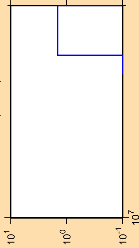
\Delta\sigma/\sigma vs. E for ^{150}\text{Gd} (mt 34)
