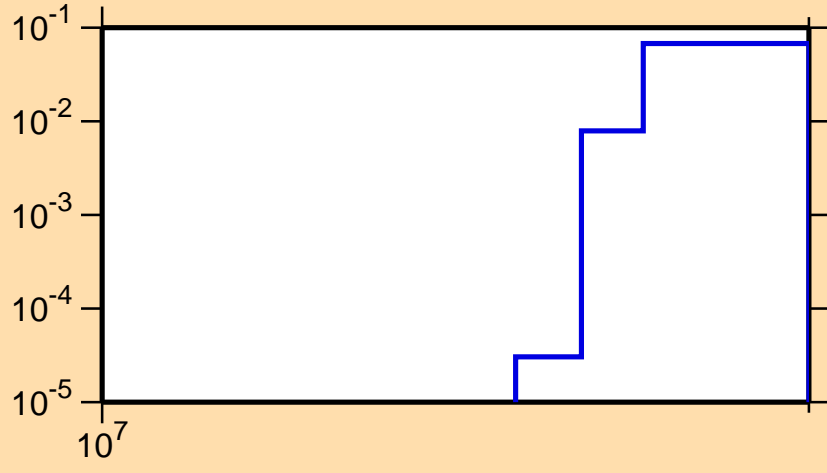
\sigma vs. E for ^{150}\text{Gd}(n,3n)
