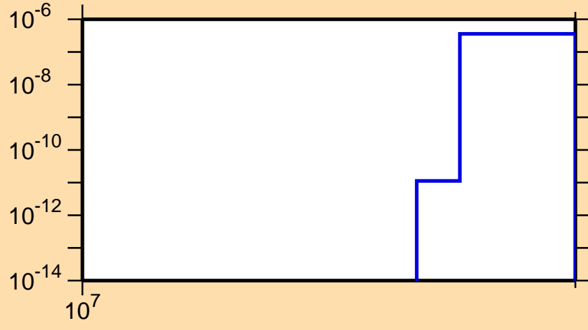
\sigma vs. E for ^{150}\text{Gd}(n,2np)
