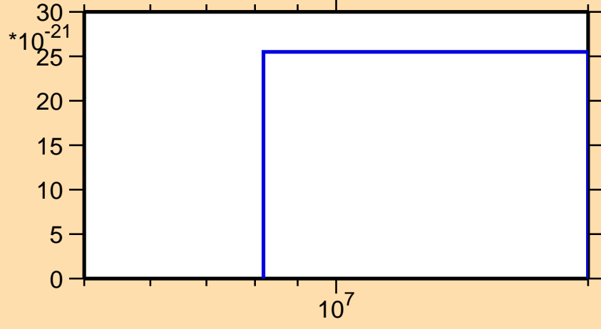
\sigma vs. E for ^{150}\text{Gd}(\text{mt } 11)
