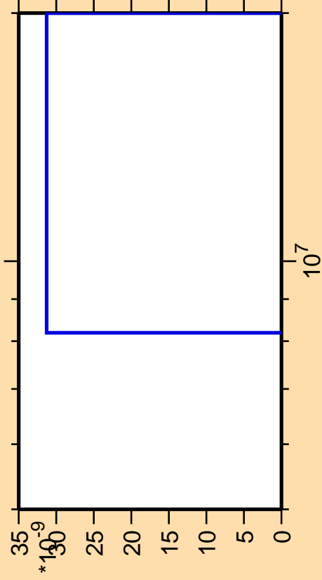
\Delta\sigma/\sigma vs. E for ^{150}\text{Gd}(\text{mt } 11)
