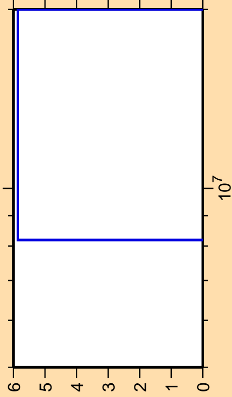
\Delta\sigma/\sigma vs. E for ^{150}\text{Gd}(n,2n)
