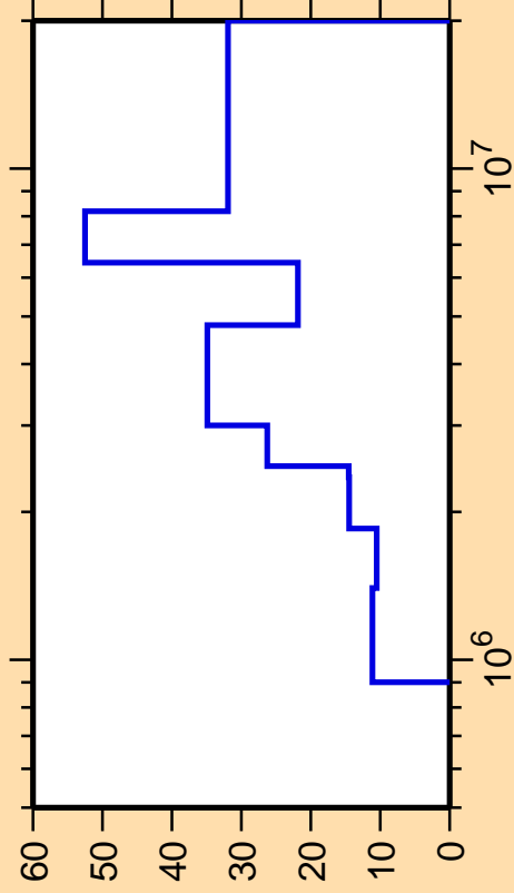
\Delta\sigma/\sigma vs. E for ^{150}\text{Gd}(n,n_3)
