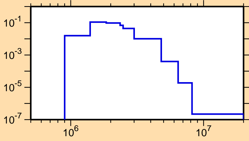
\sigma vs. E for ^{150}\text{Gd}(n,n_3)
