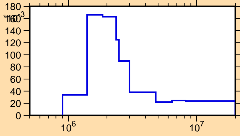
\sigma vs. E for ^{150}\text{Gd}(n,n_2)
