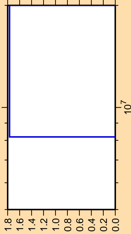
\Delta\sigma/\sigma vs. E for ^{150}\text{Gd}(n,pd)
