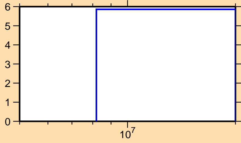
\Delta\sigma/\sigma vs. E for ^{150}\text{Gd}(n,2n)
