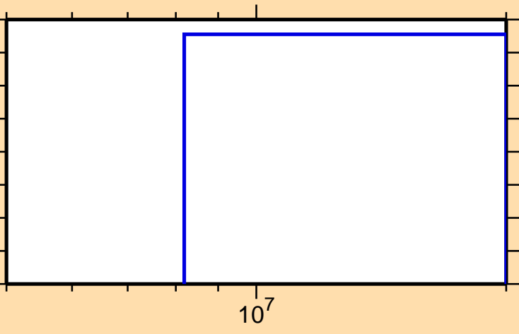
\sigma vs. E for ^{150}\text{Gd}(n,\text{pt})
