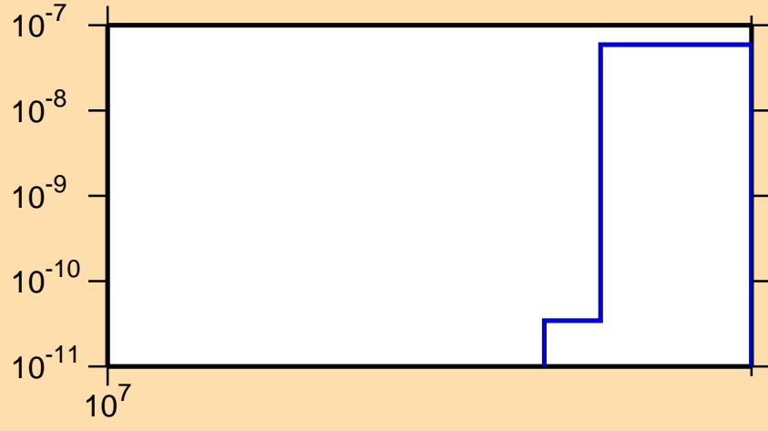
\sigma vs. E for ^{151}\text{Gd}(n,nt)
