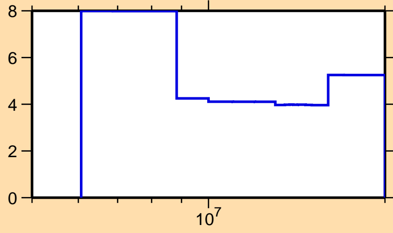
\Delta\sigma/\sigma vs. E for ^{151}\text{Gd}(n,2n)
