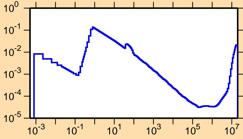
\sigma vs. E for ^{151}\text{Gd}(n,\alpha)
