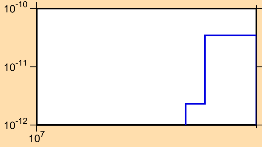
\sigma vs. E for ^{151}\text{Gd} (mt 45)
