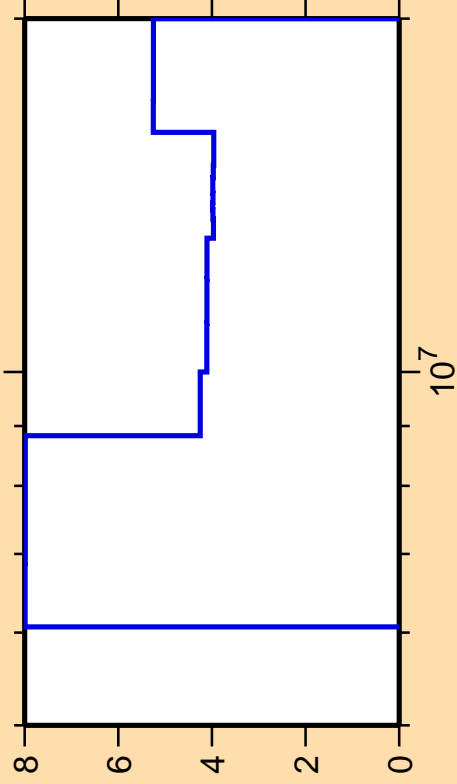
\Delta\sigma/\sigma vs. E for ^{151}\text{Gd}(n,2n)
