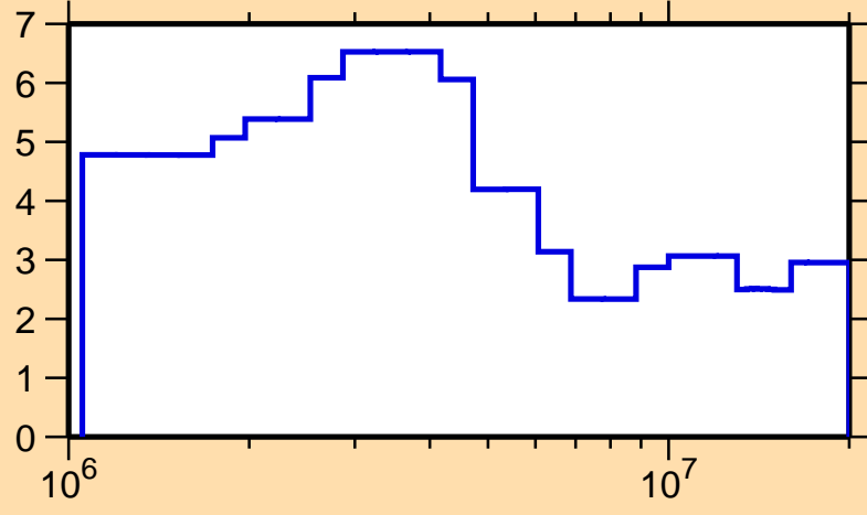
\Delta\sigma/\sigma vs. E for ^{151}\text{Gd}(n,\text{el.})
