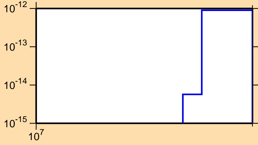
\sigma vs. E for ^{151}\text{Gd}(n,\text{pd})
