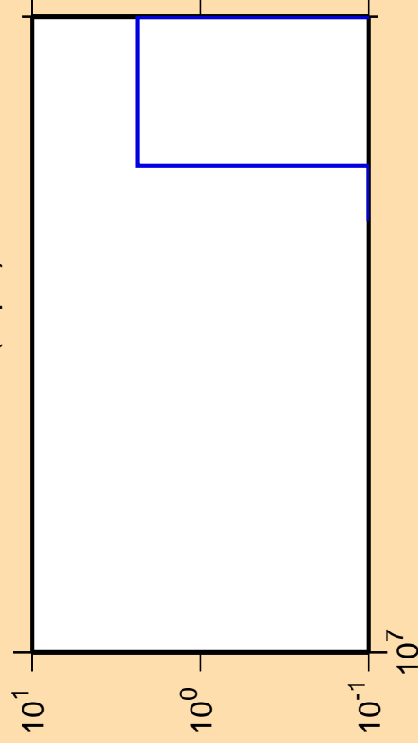
\Delta\sigma/\sigma vs. E for ^{151}\text{Gd}(n,\text{pd})
