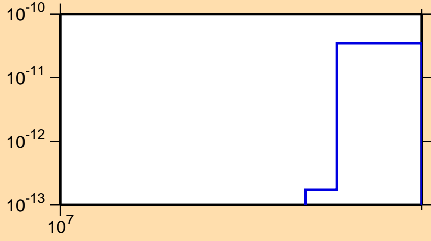
\sigma vs. E for ^{151}\text{Gd}(n,\text{pt})
