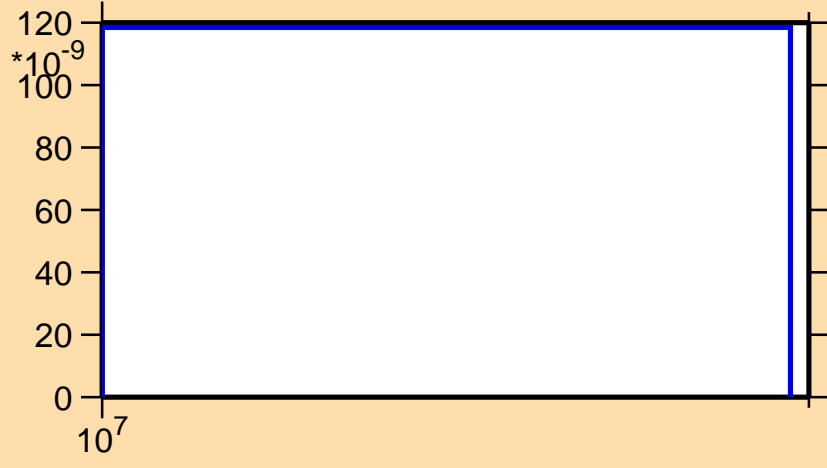
\sigma vs. E for ^{151}\text{Gd}(n,nd)
