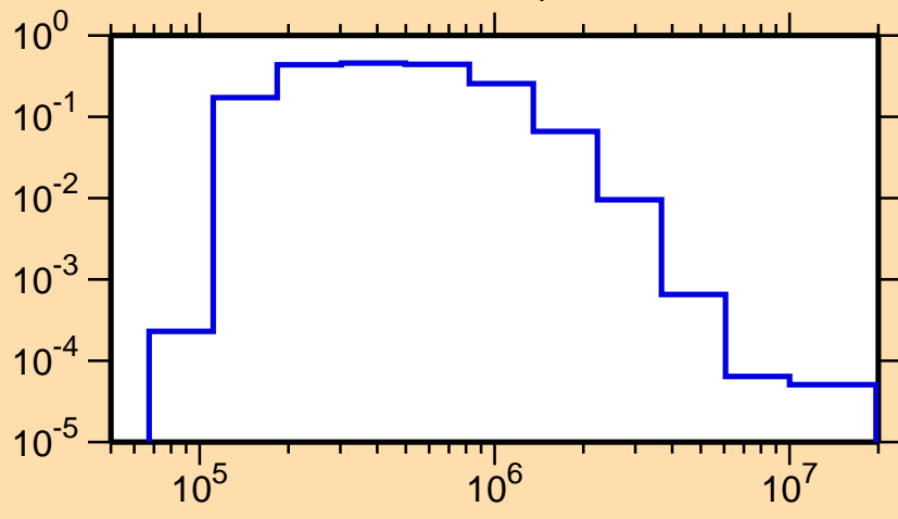
\sigma vs. E for ^{151}\text{Gd}(n,n_1)
